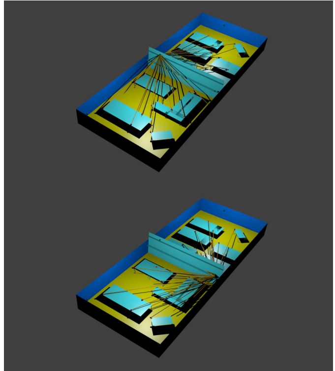
Fig. 7. UWB links evaluated by the 3D connectivity engine
