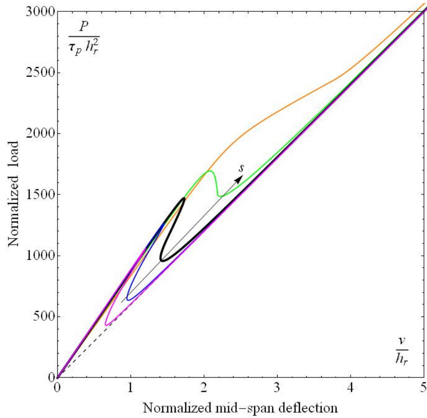
Figure 17. Load vs. mid-span deflection (dimensionless plot): size effect. The curves are plotted for brittleness number s_E = G_c/(\tau_p h_r) equal to 0.015, 0.03, 0.06, 0.12, 0.24, corresponding to a size range of 1:16. The thick line is the reference case ( s_E = 0.06 ). Note that s is inversely proportional to the structural size.
