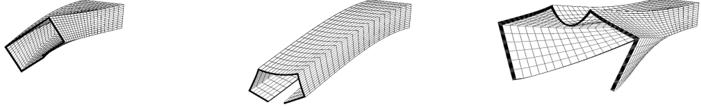
(a) Torsional mode, Freq.= 174.851 Hz (b) Bending mode, Freq.= 186.97 Hz (c) Opening mode, Freq.= 551.39 Hz
