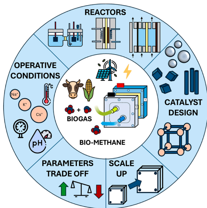
Fig. 13. Conceptual representation of the factors influencing the development of electrochemical biogas upgrading. At the core, the process couples biogas upgrading with electrochemical \text{CO}_2 conversion, offering the advantage of being directly powered by renewable electricity, thus enabling carbon-neutral or even carbon-negative energy cycles. Surrounding this central concept are the main aspects that must be addressed to achieve industrial viability: (i) catalyst and electrode design, ensuring high activity, selectivity, durability and scalability; (ii) reactor engineering and configuration, including mass transport optimization, cell architecture; (iii) operating conditions, such as pressure, temperature, electrolyte management; (iv) trade-offs among key performance indicators; (v) scaling strategies, considering techno-economic feasibility, modularity, and system robustness.
