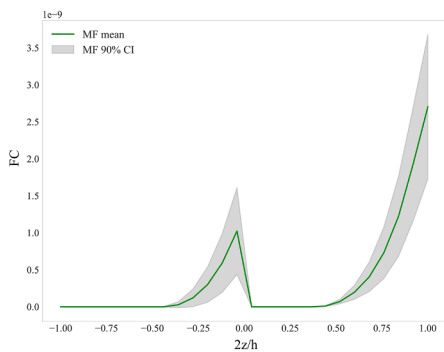
(e) FC - GPR-MF non-adaptive.
