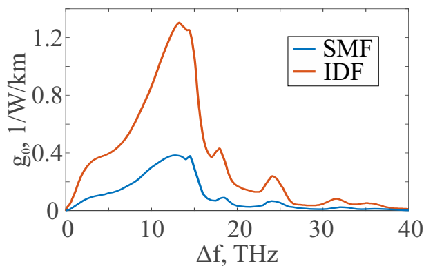
Fig. 8. The reference Raman gain coefficient, g_0 , corresponding to the Raman gain at a reference frequency, f_{ref} = 203.9 THz, for the two fibers used within this work, as a function of frequency.
