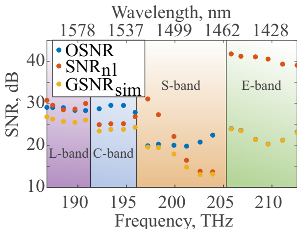
Fig. 11. The OSNR, SNR_{NL} , and GSNR_{SIM} values after propagation and amplification using the combined SCL-band Raman and the E-band BDFFA.
