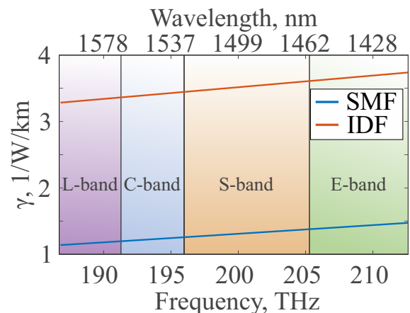
Fig. 7. The nonlinear coefficient, \gamma of SMF and IDF as a function of frequency in the ESCL-bands.
