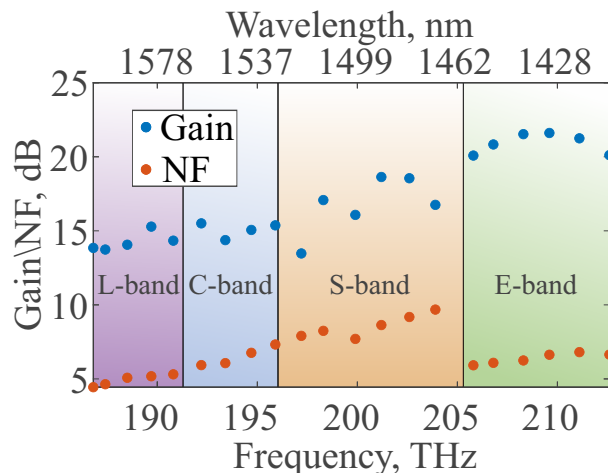
Fig. 9. The gain and NF profiles for the entire spectrum considered within the amplifier model.
