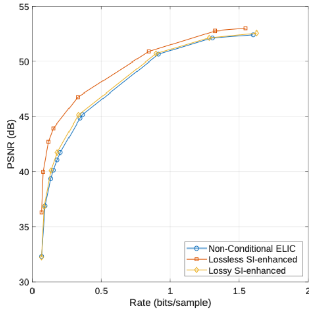
Fig. 3. Rate-distortion performance of conditional ELIC on WorldStrat using the second-to-last acquisition as SI at different quality levels.
