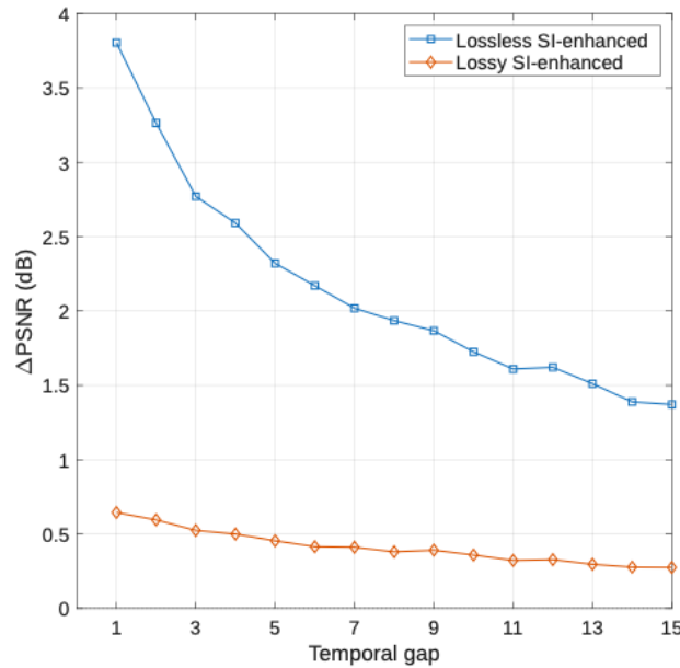
Fig. 4. Sensitivity to side-information recency, measured as the PSNR difference with respect to plain ELIC at the same operating point, as a function of the side-information acquisition time.
