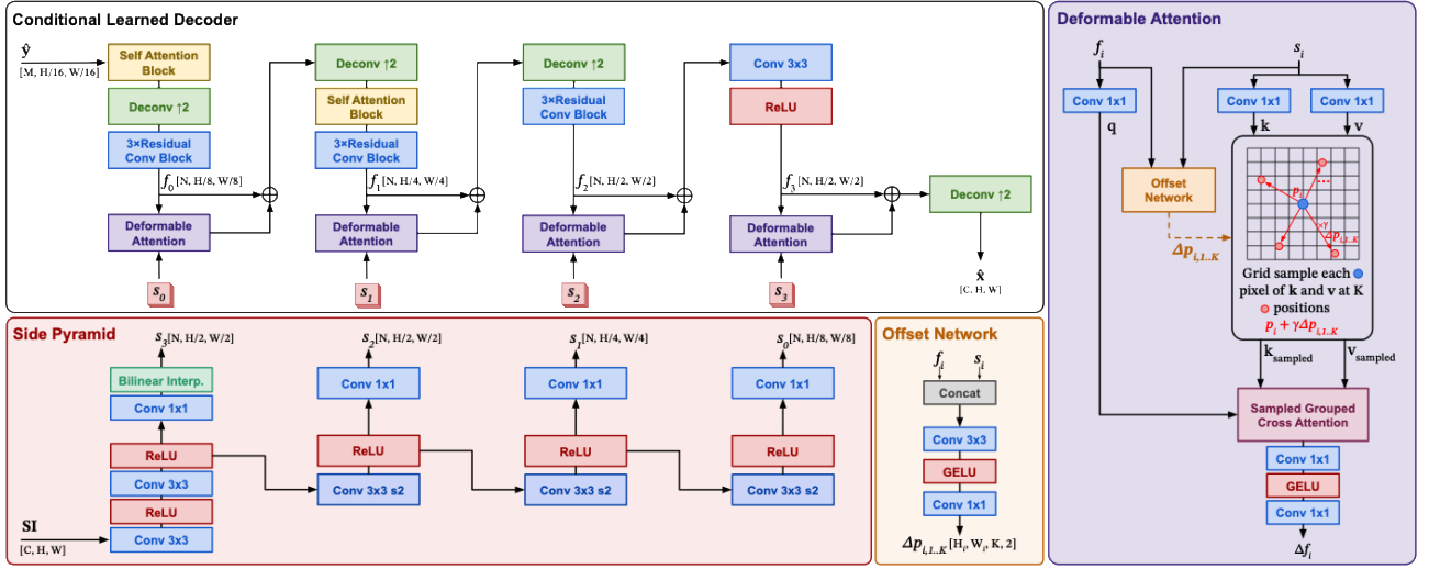
Fig. 2. Multiscale SI adapter used to inject temporal-reference features into the learned decoder.
