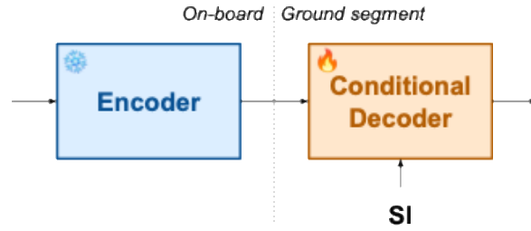
Fig. 1. Overview of the proposed conditional reconstruction . It employs a learned encoder and a conditional decoder that exploits the side information during image reconstruction.
