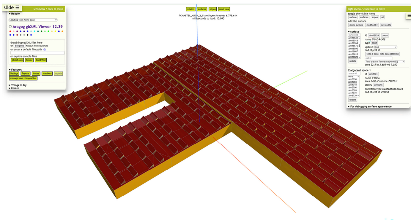
Figure 7. gbXML model of the industrial plant developed for energy analysis. The model was checked using the open-source Spider gbXML Viewer v12 by LadybugTools ( https://www.ladybug.tools/spider/gbxml-viewer/r12/gv-app/gv-app.html (accessed on 30 July 2025)).
