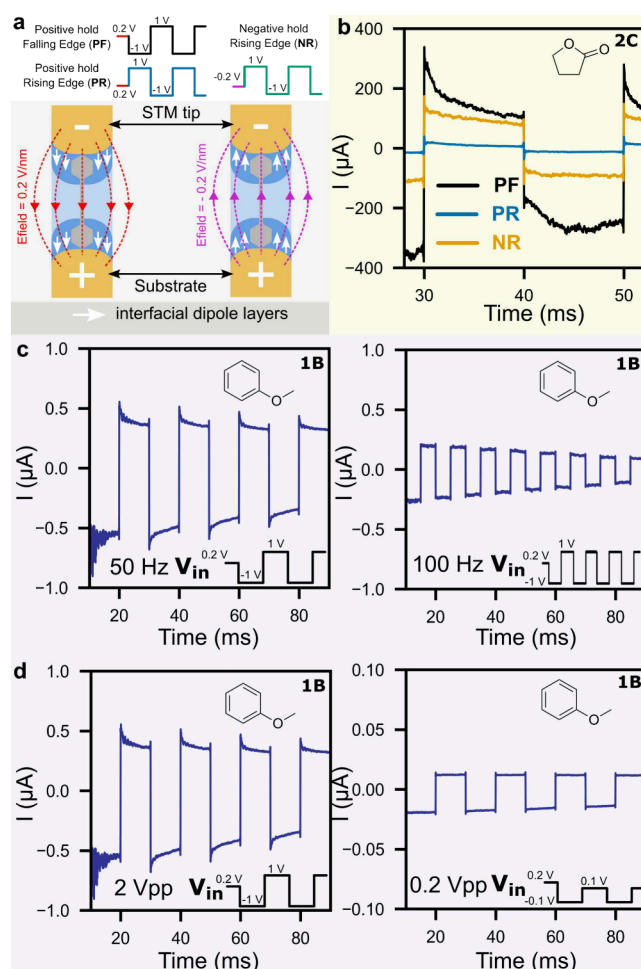
Figure 4. (a) Sketch of the initial-condition tests used to probe the origin of the nonlinear response seen in Group C solvents. We set the interfacial dipole layers (white arrows) into two opposite starting orientations by imposing an initial field of +0.2 V/nm (left) or –0.2 V/nm (right) across the tip–substrate gap, then drive the junction with the square-wave excitation sketched above each electrode pair. (b) Initial-state dependence measured in \gamma -butyrolactone, which rules out electrode asymmetry as the source of the dominant nonlinearity. The magnitude of the nonlinear response follows the excursion of the first driving edge: a larger rising or falling edge yields both a stronger nonlinearity and a larger current integrated over the full excitation period. (c, d) Frequency-dependence test in anisole, showing transition from a Group B charge/discharge behavior at 50 Hz (c) to a near-square trace typical of Group A solvents at 100 Hz (d). (e, f) Amplitude-dependence test in anisole, isolating the role of field strength in the interfacial reorganization. Reducing amplitude from 2 V_{pp} (e) to 0.2 V_{pp} (f) suppresses the transient response (note the rescaled current axis: the modulation falls to a few tens of nA and simply follows the bias), which confirms that the charging/discharging of the interfacial layers depends on the applied field strength.
