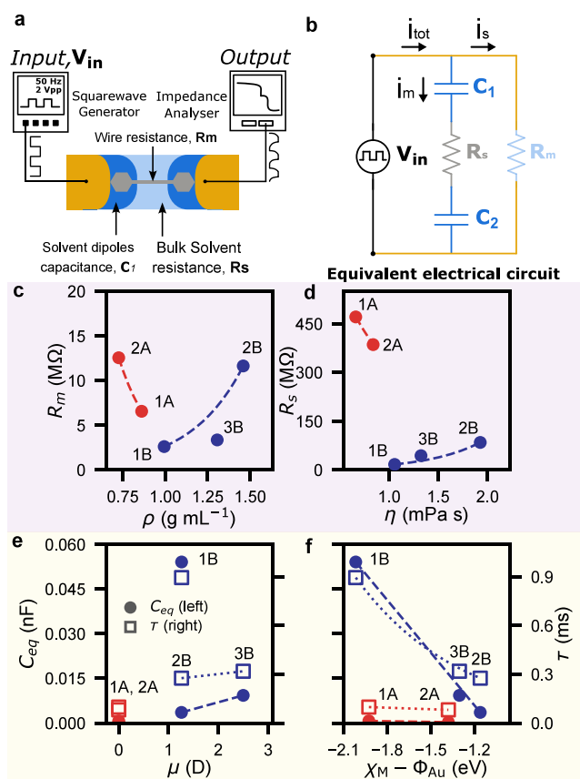
Figure 3. (a) Schematic of the AC-STMBJ experiment, showing the electrical association of each physical element: the molecular wire resistance R_m , the interfacial capacitances C_1 and C_2 arising from solvent dipolar layers, and the bulk solvent resistance R_s . (b) Equivalent electrical circuit of the SMJ in solution, with the total current dividing between the molecular branch and the interfacial branch. (c) Molecular wire resistance R_m as a function of the solvent density. (d) Solvent resistance R_s (see main text for interpretation of this value) as a function of the solvent viscosity. (e) Equivalent capacitance C_{eq} (filled circles, left axis) and the time constant \tau (open squares, right axis) as a function of the molecular dipole moment. (f) The same two quantities as a function of \Delta\chi = \chi_M - \Phi_{Au} , the difference between the Mulliken electronegativity of the solvent molecule and the work function of gold. In panels (c)–(f) red denotes Group A and blue Group B, and solvents are identified by the group codes of Figure 1c. Dashed and dotted lines are Theil-Sen guides to the eye, fitted to each group separately. Panels (c,d) and (e,f) are shaded differently only to separate the resistive from the capacitive parameters.
