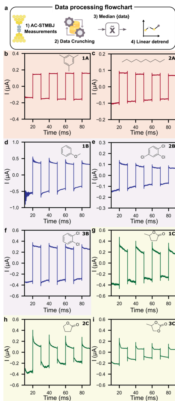
Figure 2. (a) Flowchart of the AC-STMBJ data processing pipeline: acquisition of the raw traces, data crunching, trace-by-trace median extraction, and linear detrending. (b–i) Representative single current traces measured in the investigated solvents: mesitylene, decane, anisole, 1,2,4-trichlorobenzene, 1,2-dichlorobenzene, \gamma -valerolactone, \gamma -butyrolactone, and propylene carbonate.
