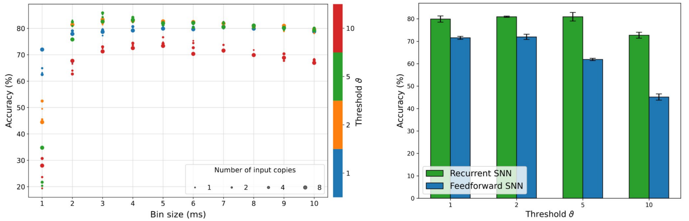
Fig. 7. Summary of the accuracy performances of RSN and FFSNN resulting from the grid search exploration in the two-step HPO procedure. (a) Best test accuracy results achieved with the RSN for all the combinations of time_bin_size and nb_input_copies . (b) Mean and standard deviation of the accuracy results of both the FFSNN and the RSN with the best parameters for each encoding threshold.
