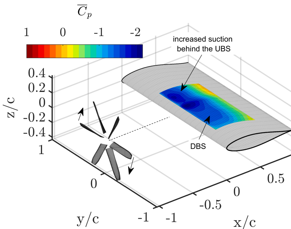
Fig. 10. Time-averaged pressure coefficient ( \bar{C}_p ) distribution obtained from the pressure sensors. Wing at \alpha = 6^\circ and propeller with \beta_{\frac{z}{r}} = 0.7 = 30^\circ operating at J = 0.8 .
