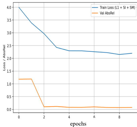
Figure 3. The trend of Train Loss and AbsRel of second step
