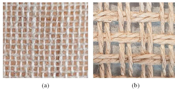
Fig. 1. Flax textile reinforcements adopted in the present study: (a) “K” and (b) “F” textiles.
