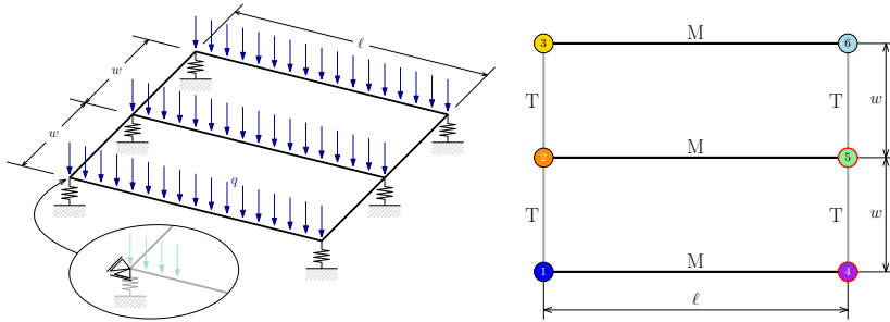
Fig. 1 Sketch of the reference grillage.
