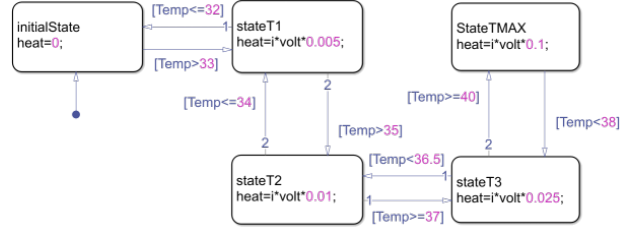
Fig. 2. The inner structure of the thermal model state flow chart.
