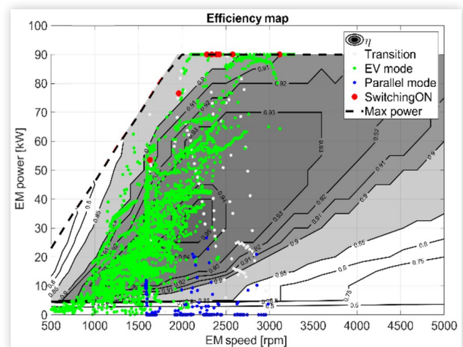
FIGURE 8 RDE 1 —EM working points in speed (x-axis) power (y-axis) map and full-load curve. Green dots: EV mode; blue dots: parallel mode; red dots: engine switching on; gray dots: transition phases, i.e., the engine status and the clutch engagement are changing.
