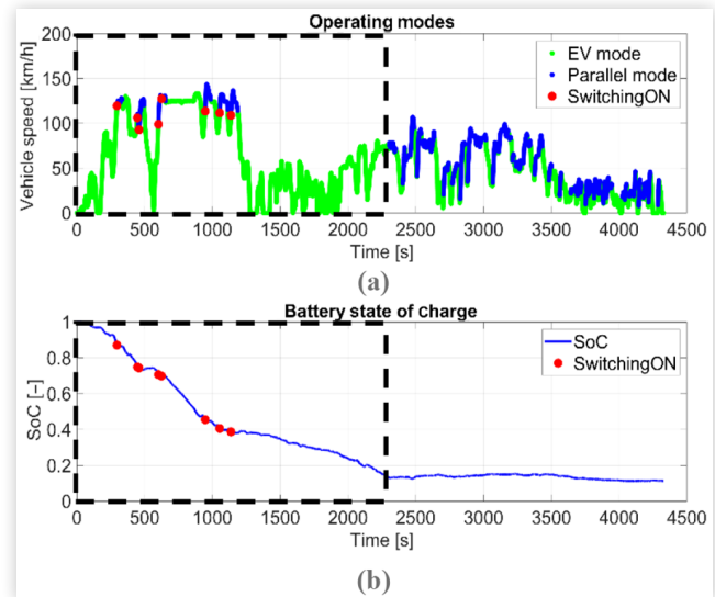
FIGURE 7 RDE 1 . (a) Vehicle speed profile along with the operating modes: EV mode (green) and parallel mode (blue); (b) Battery SoC profile in the function of time. The dashed area highlights the section performed in CD mode. The ICE switching on during the CD phase is denoted with red dots.
