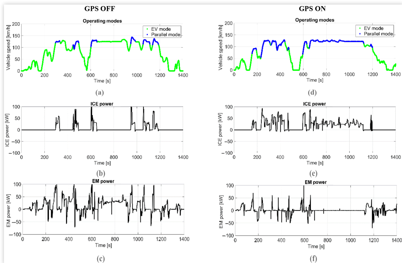
FIGURE 20 Power split during the highway section: RDE_1 (on the left) and RDE_2 (on the right) with the navigation system disabled and enabled, respectively.
