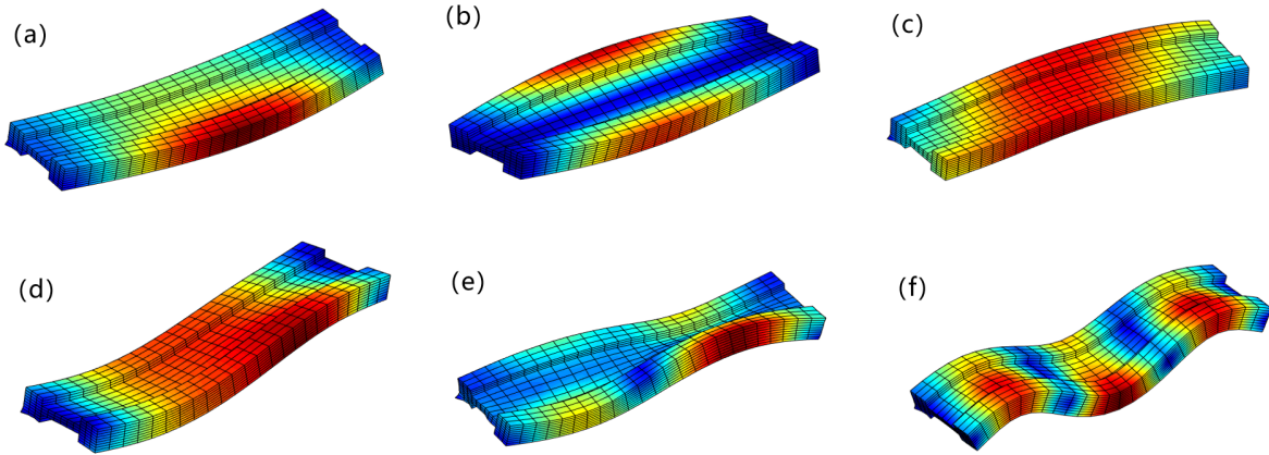
Fig. 15. Flexural (a,c,d,f) and shell-like (b,e) modal shapes for a SS stiffened panel structure ( L = a_1 \times 15 ), 8L9.
