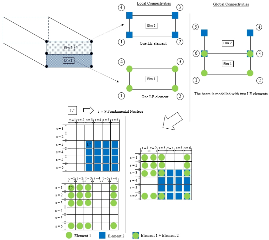
Fig. 4. Expansion of the matrix \mathbf{L}^{\tau s} for two L4 elements assemblies within a beam node.
