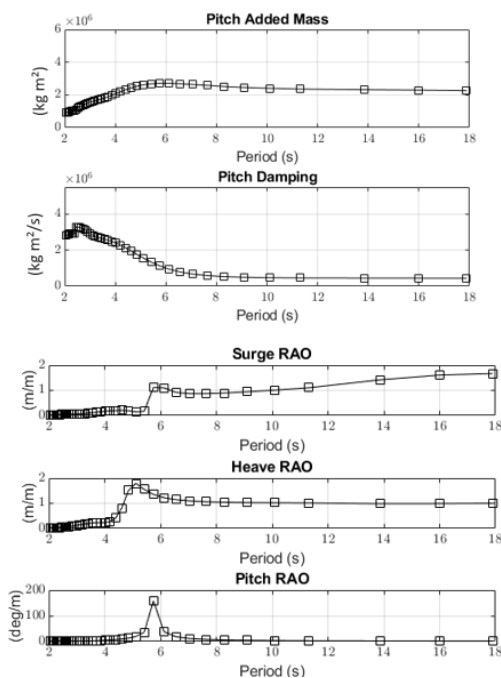
FIGURE 12: Pitch added mass, radiation damping and RAOs for the spline-based hull.
