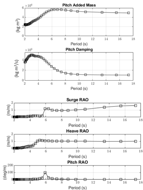
FIGURE 11: Pitch added mass, radiation damping and RAOs for the arc-based hull.
