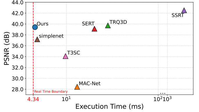
Fig. 3: Runtime on Nvidia Jetson Orin Nano normalized for a 1 \times 1000 \times 66 line. 4.34ms is the Line Acquisition Time of the PRISMA satellite.
