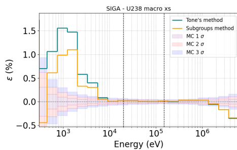
(c) \Sigma_a macroscopic cross section for ^{238}\text{U} .
