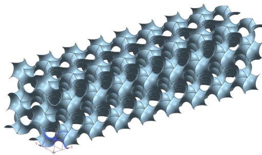
Figure 5. Square section channel filled with a fluid-saturated engineered metal foam based on gyroid TPMS [46].
