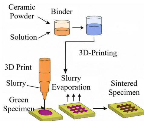
FIGURE 3 | Schematic of making a manufactured part using the extrusion method.
