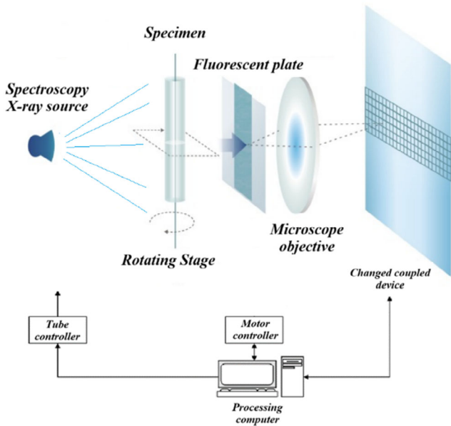
FIGURE 30 | Schematic of micro-computed tomography ( \mu -CT). Reproduced with permission [268]. Copyright 2012, IntechOpen.
