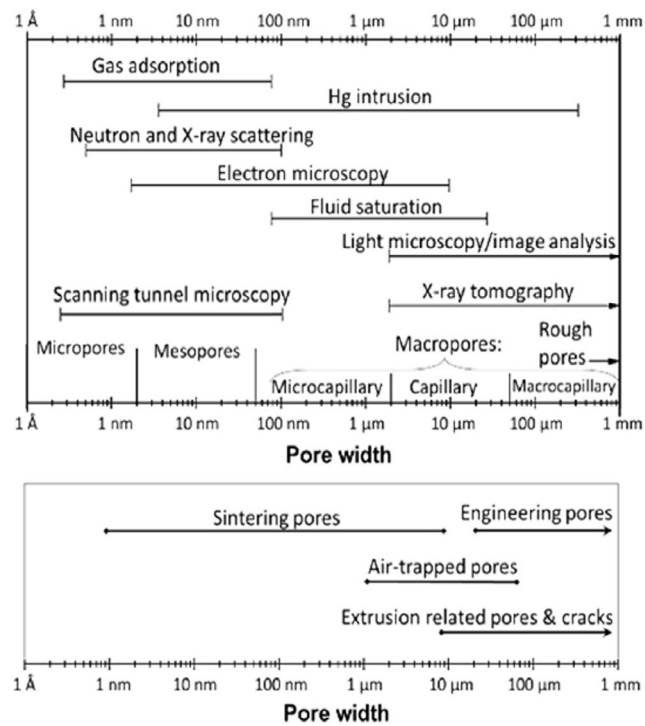
FIGURE 28 | Investigation of porosities and defects length in EAM ceramics. Reproduced with permission [37]. Copyright 2021, Elsevier.
