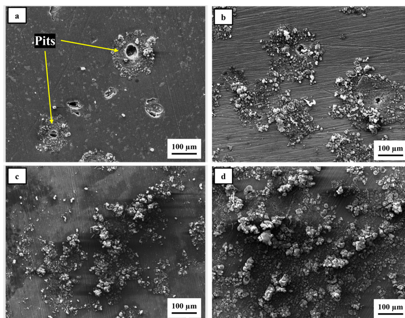
Figure 10. SEM images of the sample surfaces after the potentiodynamic polarization test: (a) BM, (b) SZ, (c) BM-PA, and (d) SZ-PA.
