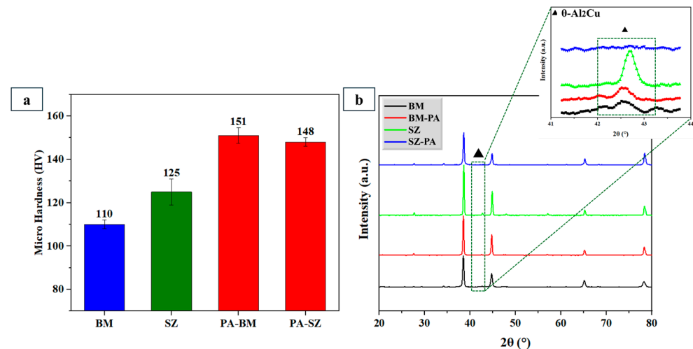
Figure 2. (a) Vickers microhardness and (b) XRD patterns of BM, SZ, BM-PA, and SZ-PA.
