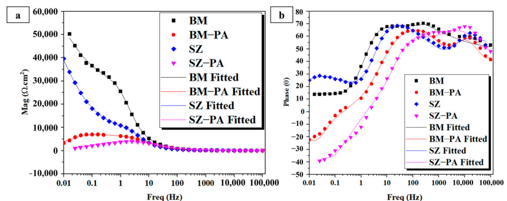
Figure 8. (a) Bode magnitude plots and (b) phase-angle plots of BM, BM-PA, SZ, and SZ-PA.
