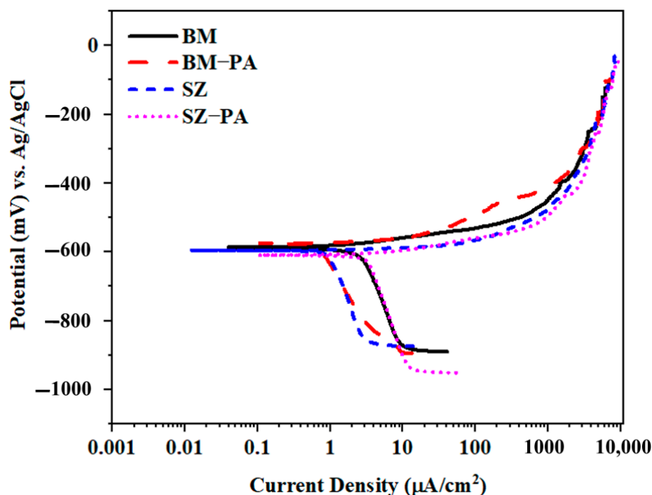
Figure 6. Potentiodynamic polarization curves for BM, SZ, BM-PA, and SZ-PA samples.
