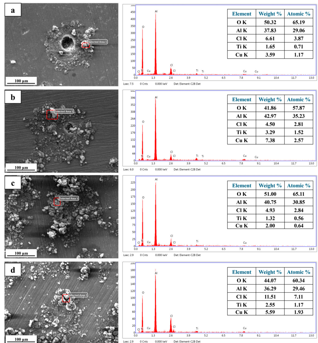
Figure 11. Representative SEM images and corresponding EDS analysis performed on the marked locations from the corroded surfaces after the potentiodynamic polarization test: (a) BM, (b) SZ, (c) BM-PA, and (d) SZ-PA.
