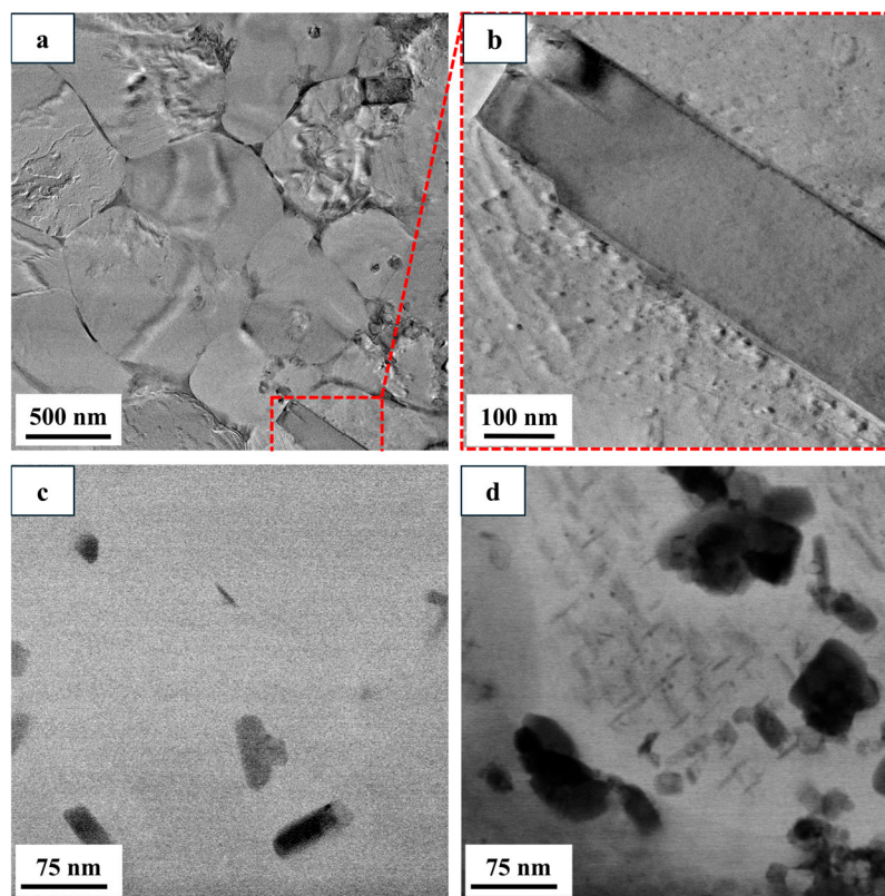
Figure 4. TEM micrographs showing the microstructure of (a) the BM, (b) a magnified view of a TiB 2 particle from (a), (c) the SZ, and (d) after solution treatment and peak-aging.
