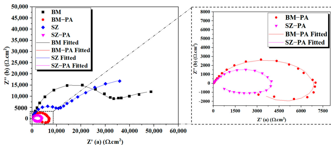
Figure 7. Nyquist plots of the EIS spectra for BM, BM-PA, SZ, and SZ-PA samples.
