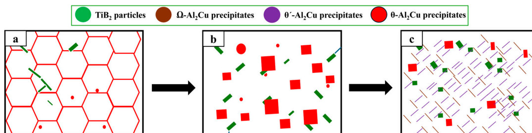
Figure 5. Schematic illustration of the microstructural evolution from (a) the BM to (b) the SZ and finally to (c) the peak-aged condition.
