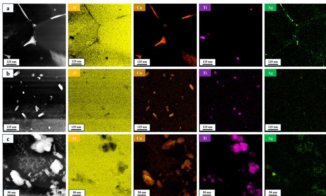
Figure 3. STEM-EDS maps showing the distribution of precipitate-forming elements in (a) BM, (b) SZ, and (c) BM-PA. Mg and Si were also detected and were distributed relatively homogeneously.
