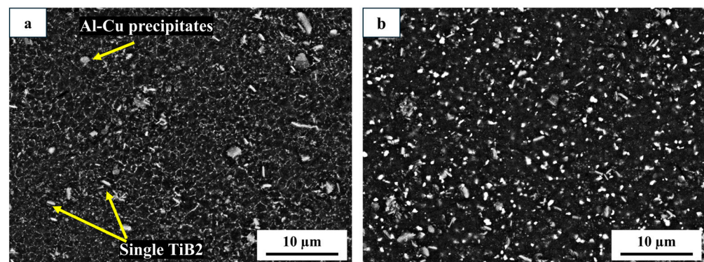
Figure 1. SEM micrographs of (a) the base material and (b) the stir zone.
