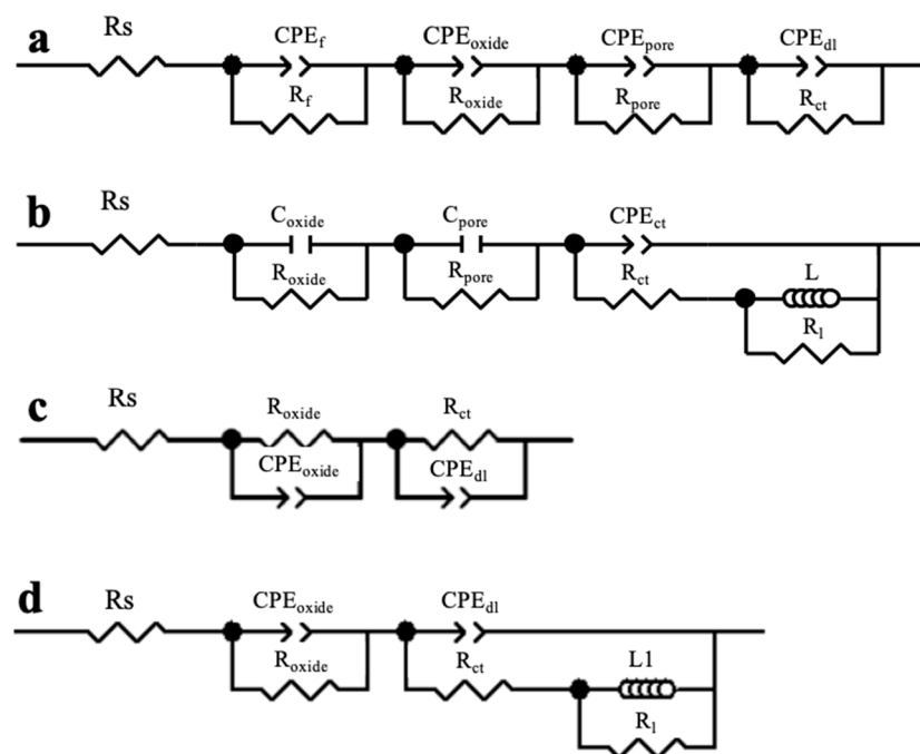
Figure 9. Equivalent electrical circuits obtained from ZView fitting for (a) BM, (b) BM-PA, (c) SZ, and (d) SZ-PA.
