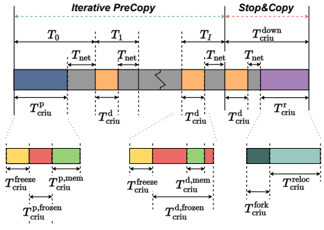
Fig. 2: Live migration diagram: CRIU implementation
