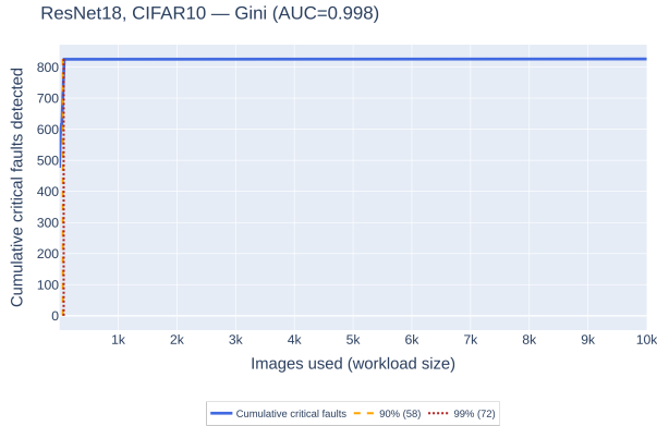
(c) Gini-Index
