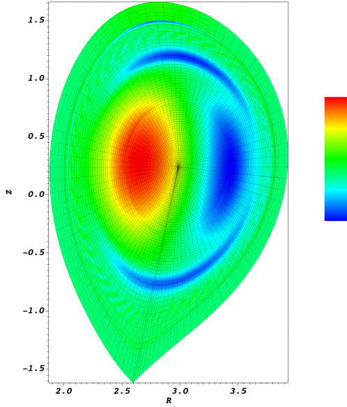
Figure 20: Perturbed pressure at t = 4.5 ms for forced oscillator frequency at resonance, f_0 = 311.5 \text{ kHz} . Overlaid is displayed the grid showing the radial grid point packing at the plasma boundary and poloidal angle grid point packing at the X-point.
