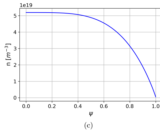
Figure 3: EFIT equilibrium pressure profile (3a), and safety factor (3b); best fit of the experimental electron density profile (3c), as functions of normalized flux. The separatrix is at \psi = 1 .
