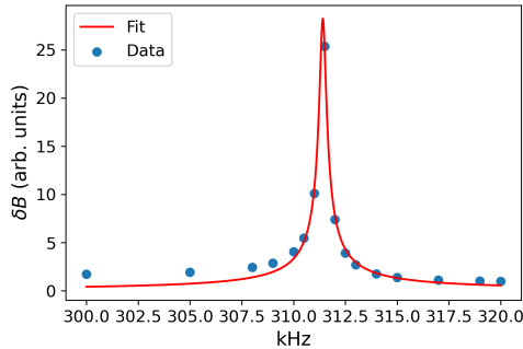
Figure 18: Normalized amplitude of the normal component of the perturbed magnetic field as a function of oscillator frequency f_0 in the neighbourhood of f_{high} . Blue dots, corresponding to numerical results, are fitted by the red curve, assuming the resonant condition (12).
