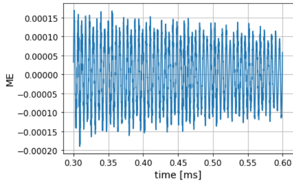
Figure 4: Oscillatory behaviour of the magnetic energy in response to a "vertical push", in the time interval between t = 0.3 ms and t = 0.6 ms.
