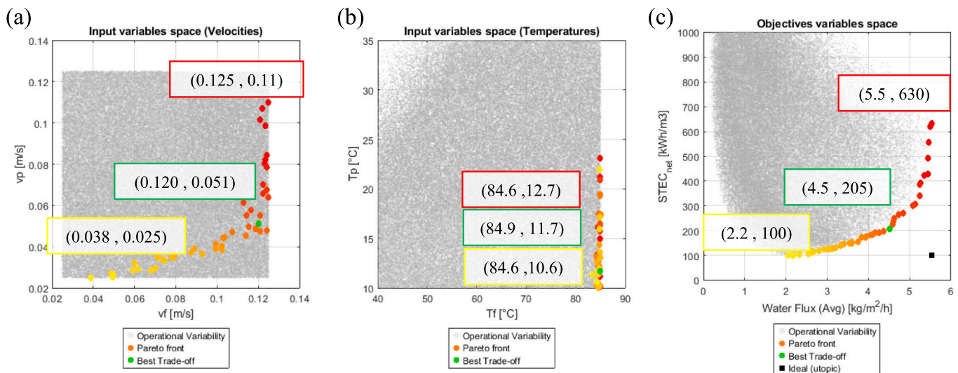
Fig. 6. The optimization identifies the Pareto Front by varying inlet velocities and temperatures to find the optimal operating conditions. (a) Input variables (velocities): shows the relationship between the optimal feed velocity ( v_{f,in} ) and permeate velocity ( v_{p,in} ). (b) Input variables space (temperatures): shows the relationship between the optimal feed inlet temperature ( T_{f,in} ) and permeate inlet temperature ( T_{p,in} ). (c) Objectives variables: The resulting Pareto Front illustrating the trade-off between average water flux and net STEC. Three operational conditions are selected for analysis, highlighted in boxes (red, green and yellow), described also in Table 3. (For interpretation of the references to colour in this figure legend, the reader is referred to the web version of this article.)
