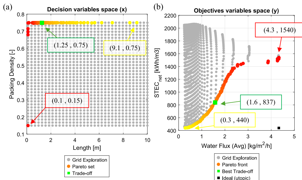
Fig. 5. Results of the initial optimization stage identifying the optimal structural configuration for the DCMD module. In Fig. 5b, each point represents expected/average values over 100 Monte Carlo realization. The optimization, considering length and packing density as decision variables, reveals the pareto front showing the compromise between water flux and net STEC. Three designs are selected for analysis, highlighted in boxes (red, green and yellow), described also in Table 2. (For interpretation of the references to colour in this figure legend, the reader is referred to the web version of this article.)
