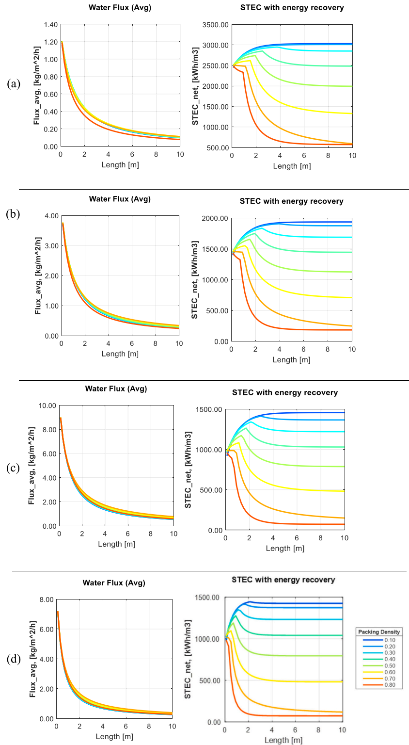
Fig. 4. Effect of contact length on various parameters at different values of packing densities varied from 0.1 to 0.8. (a) Feed and permeate inlet velocities 0.1 m/s each, feed inlet temperature 40 °C, permeate inlet temperature 25 °C. (b) Feed and permeate inlet velocities 0.1 m/s each, feed inlet temperature 60 °C, permeate inlet temperature 25 °C. (c) Feed and permeate inlet velocities 0.1 m/s each, feed inlet temperature 80 °C, permeate inlet temperature 25 °C. (d) Feed and permeate inlet velocities 0.05 m/s each, feed inlet temperature 80 °C, permeate inlet temperature 25 °C.
