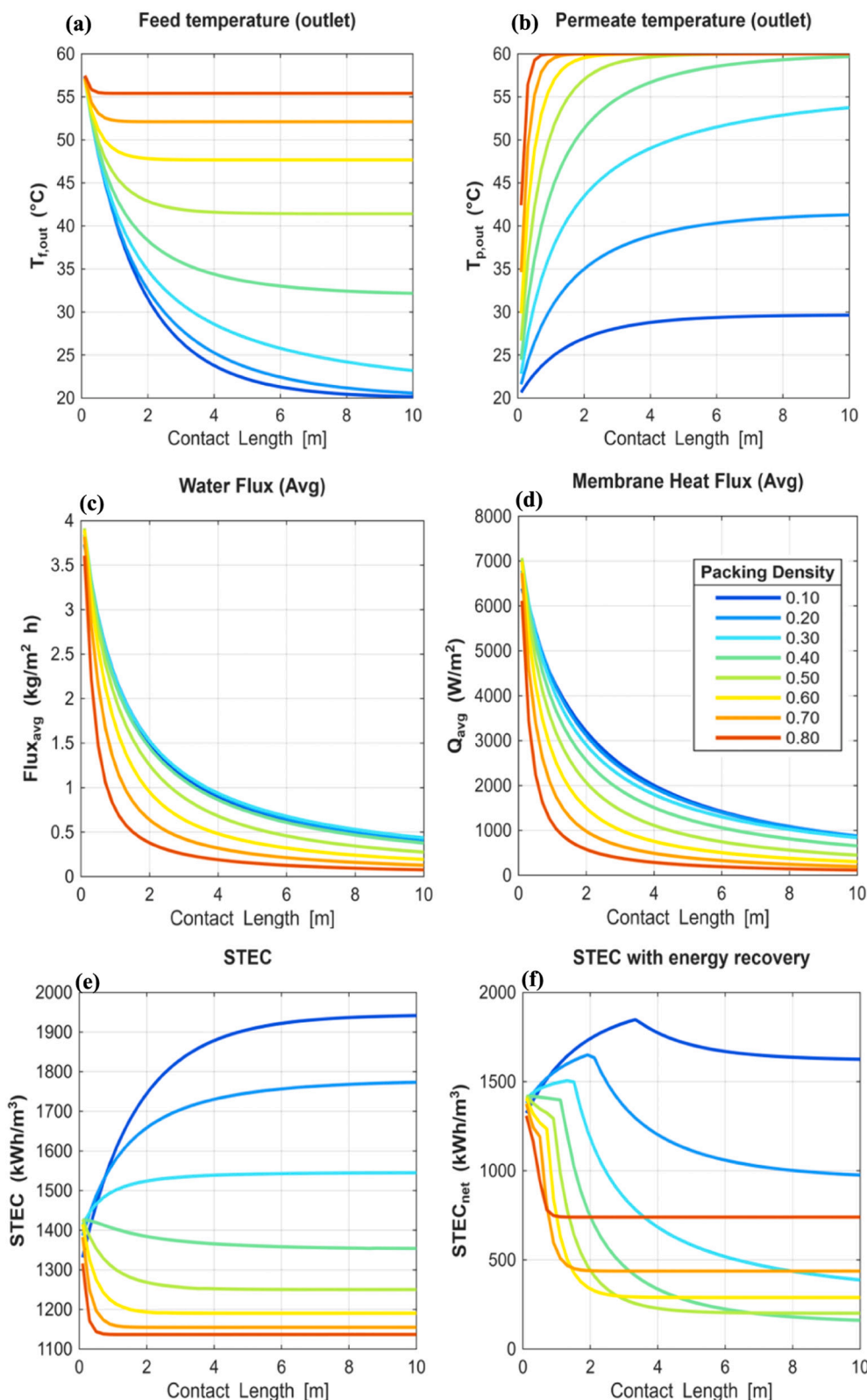
Fig. 3. Effect of contact length on various parameters at different values of packing densities ranging from 0.1 to 0.8. The operating conditions were set at: inlet feed temperature 60 °C, inlet permeate temperature 20 °C, inlet feed velocity 0.125 m/s and inlet permeate velocity 0.025 m/s.
