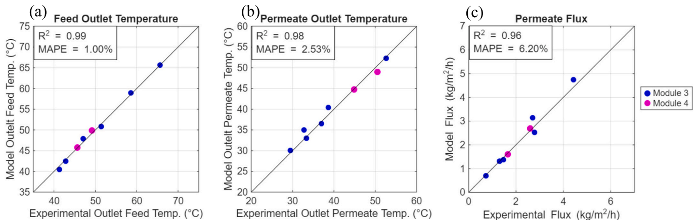
Fig. 7. Experimental validation of the DCMD model using membrane Modules 3 and 4 under different operating conditions: comparison between experimental and predicted values of (a) feed outlet temperature, (b) permeate outlet temperature, and (c) permeate flux. The solid line represents perfect agreement between model predictions and experimental data.
