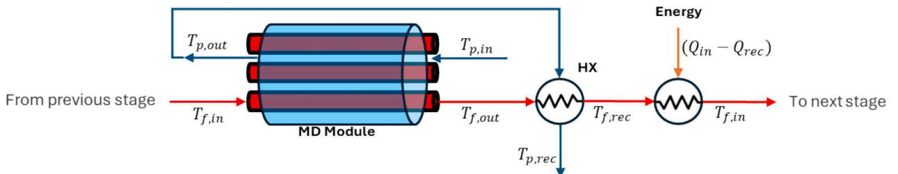
Fig. 1. Energy recovery strategy.
