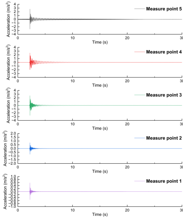
(b) Time-history signal of damage condition scale model
