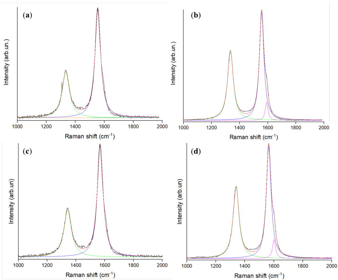
Figure S1: Fitted D and G peak of a) fresh 0CNT, b) fresh 60CNT, c) spent 0CNT, and d) spent 60CNT.
