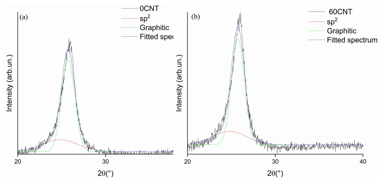
Figure S2: Fitted XRD patterns of a) fresh 0CNT and b) fresh 60CNT.
