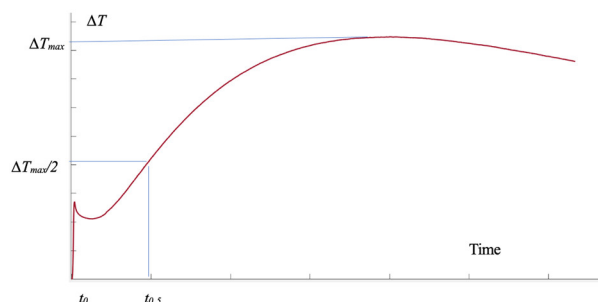
Figure 2. Transient temperature curve of a specimen after light pulse heating [19].
