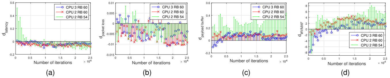
Fig. 13. Performance of VERA under varying CPU and RB budget constraints: (a) latency, (b) packet loss, (c) payout buffer, and (d) WVMAF
