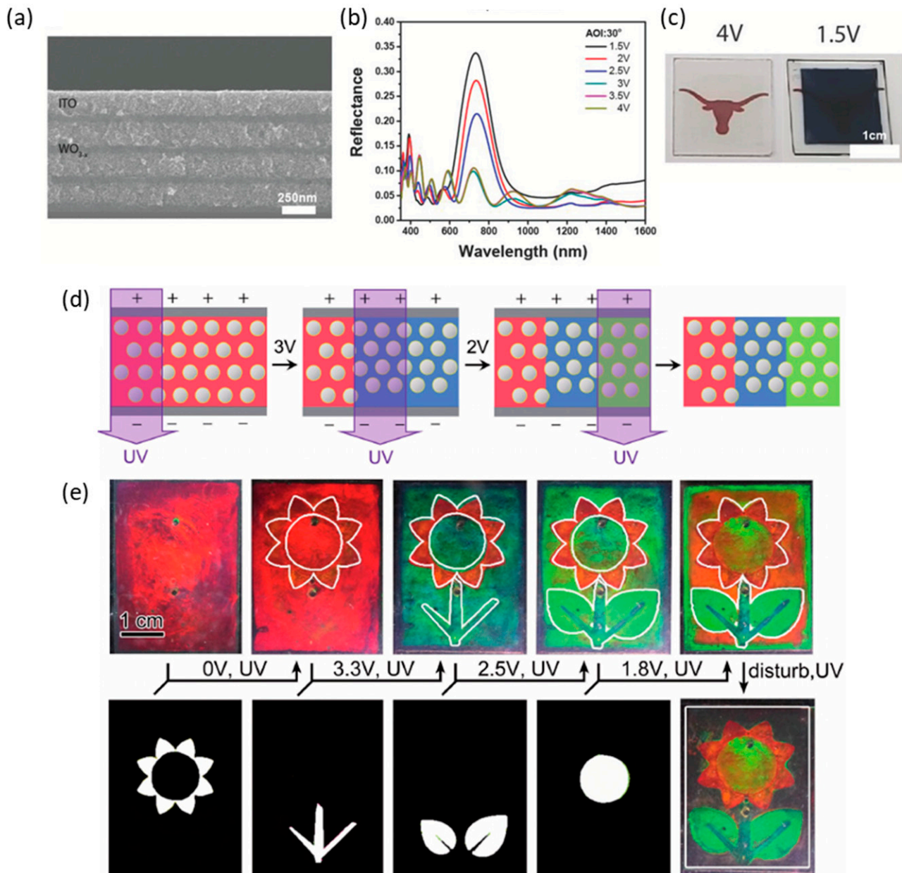
Figure 4. (a–c) Cross-sectional SEM image, reflectance spectra and optical image of 1D photonic crystals constituted of indium tin oxide (ITO) NCs and WO_{3-x} NC layers (BS1). Adapted from reference [90] under permission from John Wiley & Sons. Effect of an electric tuning and UV curing combination on E-ink. (d) Schematic mechanism and (e) optical example of lithographical printing by photomask covering. Adapted from reference [91] under permission from John Wiley & Sons.
