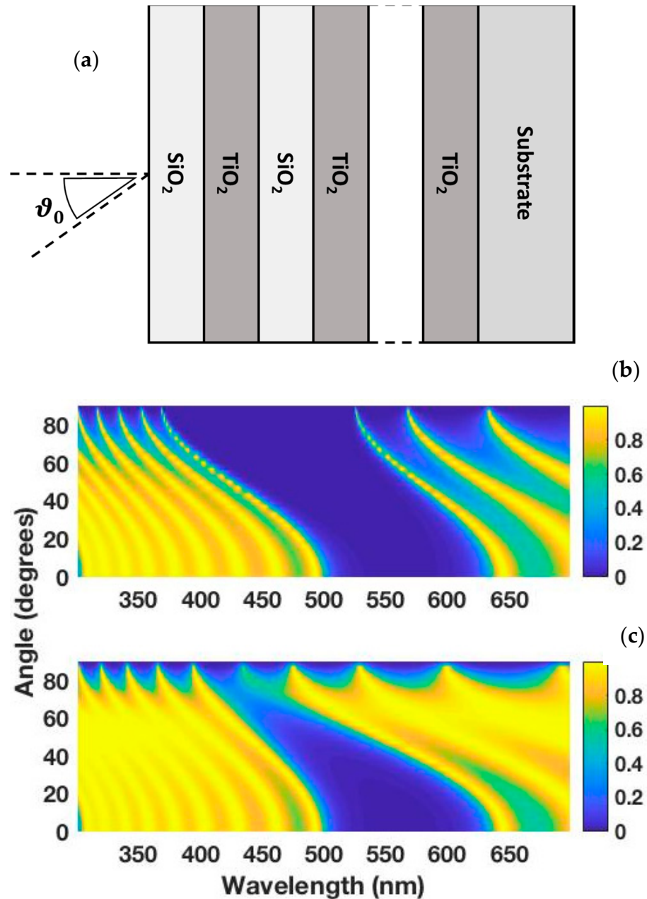
Figure 1. (a) Sketch of the one-dimensional photonic crystal ( \vartheta_0 is the angle of incidence of the light). Simulation of the angular dependent transmission spectrum of a 5 bilayer \text{TiO}_2 - \text{SiO}_2 nanoparticle-based photonic crystal for a transverse electric (TE) wave (b) and a transverse magnetic (TM) wave (c). For both the nanoparticle layers, the filling factor is 0.7.
