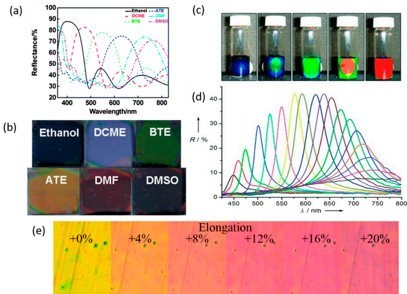
Figure 2. Different cases of tunable photonic crystals. (a,b) Reflectance spectra and visual effect of PMMA-co-PHEMA-co-PEGDMA) and titania photonic crystals (PhCs) in different solvents. Adapted from reference [32] by permission of The Royal Society of Chemistry. (c,d) Effect of the magnet–sample distance on polyacrylate-capped superparamagnetic magnetite ( \text{Fe}_3\text{O}_4 ) colloidal nanocrystal clusters (CNCs). Adapted from reference [110] by permission of John Wiley & Sons. (e) Changing of structural color of grating nanostructured polydimethylsiloxane membrane/ \text{TiO}_2 as the elongation increases. Adapted from reference [31].
