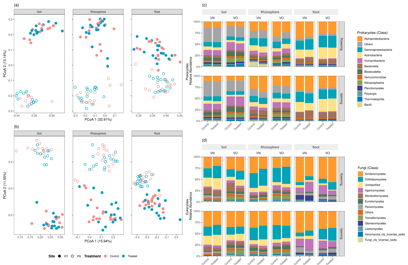
Fig. 1. Assembly and diversity of Vitis vinifera (Pigato) vineyard microbiota across compartments, stages, and treatment conditions. Prokaryotic and fungal communities were profiled in root endosphere, rhizosphere and bulk soil during the flowering and ripening phenological stage in two vineyards (sites), namely VO and VN, inoculated (treated) or not (control) with a commercial microbial inoculum. (a-b) Principal Coordinate Analysis (PCoA) plot of Bray-Curtis distances between samples by treatment of prokaryotic (a) and fungal communities (b) across the different compartments in both vineyards. Points represent single samples and are coloured by treatment. The fraction of the total variance explained by the projection is indicated in brackets along each axis. (c-d) Average relative abundances of prokaryotes (c) and fungi (d) at the class level.
