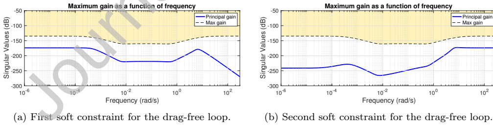
Figure 14: Soft constraints defined for the drag-free loop.
