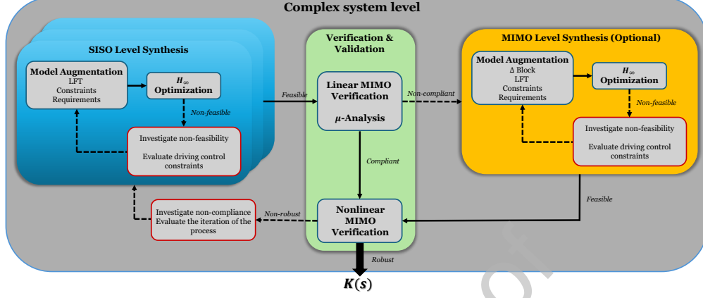
Figure 2: Closed-loop general scheme for the systematic design.
