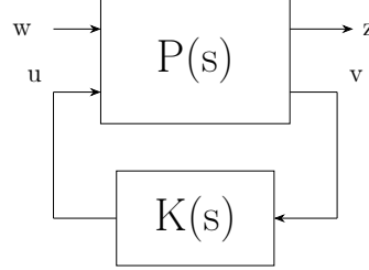
Figure 1: General lower-LFT interconnection between the generalized plant P(s) and the dynamic output-feedback controller K(s) .
