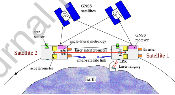
Figure 13: Low-Low Satellite-to-Satellite Tracking (LL-SST) measurement principle for the NGGM mission [35].
