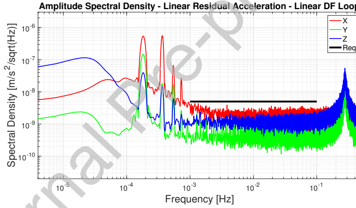
Figure 19: Amplitude Spectral Density (ASD) of the residual linear acceleration.
