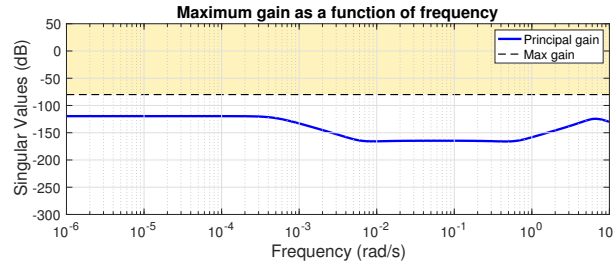
Figure 16: Hard constraint for the drag-free loop.
