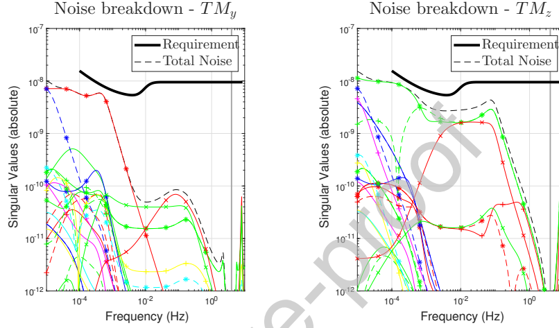
Figure 10: Noise contributions to the TM linear position.
