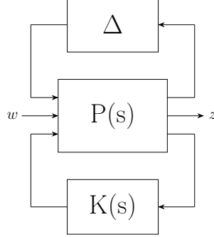
Figure 3: LFT interconnection of the system for \mu -analysis. \Delta represents the uncertainty block, P is the plant and K is the controller.
