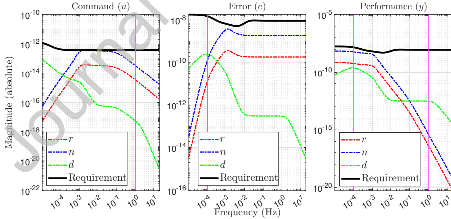
Figure 8: Contribution to the output channel for the TM suspension loop in y .
