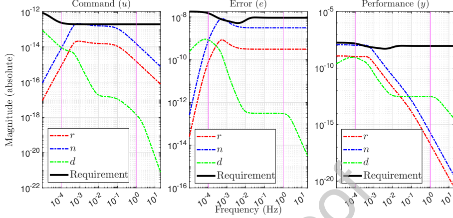
Figure 9: Contribution to the output channel for the TM suspension loop in z .
