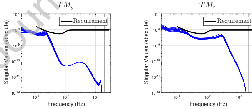
Figure 11: TM linear position singular values.
