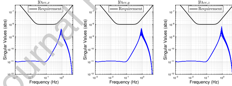
Figure 18: Worst-case performance analysis for DF loop.
