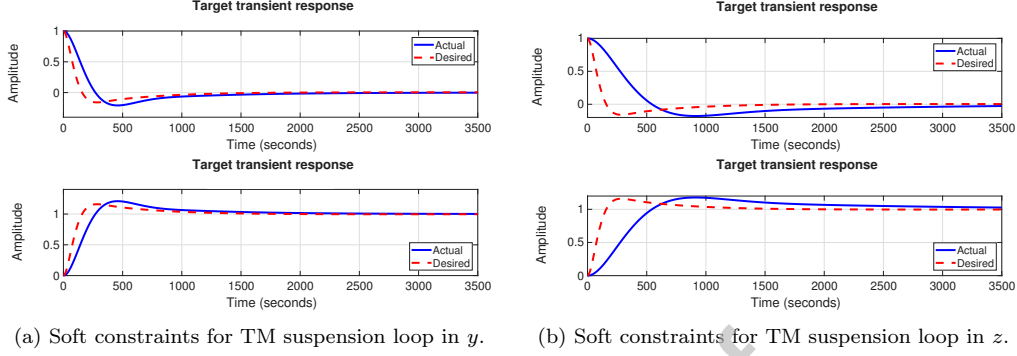
Figure 7: Soft constraints for TM suspension loop.
