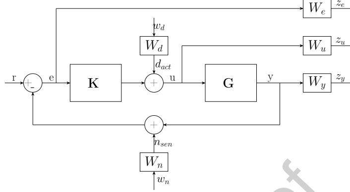
Figure 5: Generic closed-loop SISO diagram with appended weighting functions.
