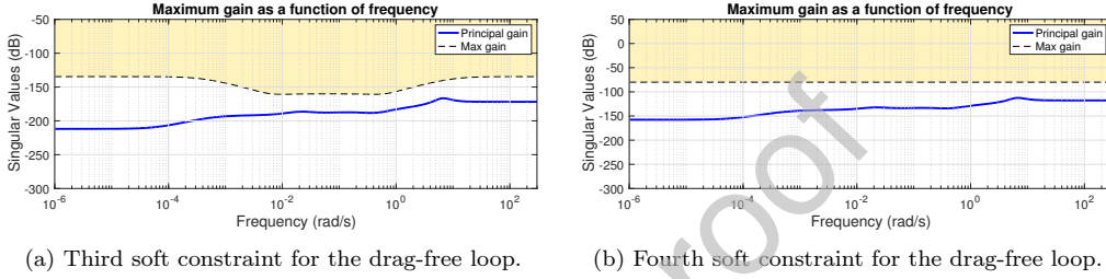
Figure 15: Additional soft constraints defined for the drag-free loop.
