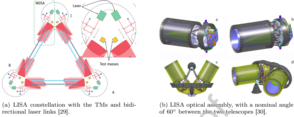
Figure 4: LISA configuration overview.
