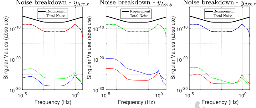
Figure 17: Noise contribution to the DF loop.
