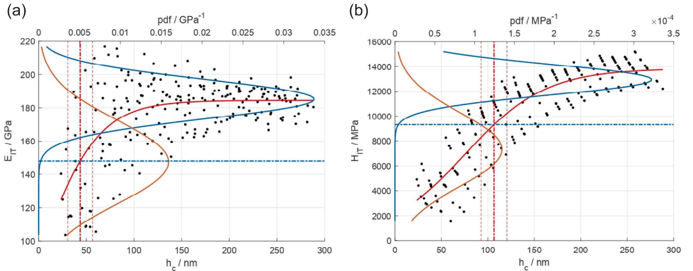
Fig. 7. Method application result for \text{ZrO}_2\text{AgNP}/\text{Si}\langle 1\ 0\ 0 \rangle with a deposition duration of 60'. Black points: measured data. Orange solid line: probability density function of the coating (transition layer) mechanical response. Blue solid line: probability density function of the substrate mechanical response. Red solid line: fitted M = g(h_c) . Blue dot-dashed line: M_2^* . Red dot-dashed line: t_c = t_{M,2}^* = g^{-1}(M_2^*) , with expanded uncertainty (95% confidence level) (red dashed lines). Deconvolution of (a) E_{IT} and (b) H_{IT} .
