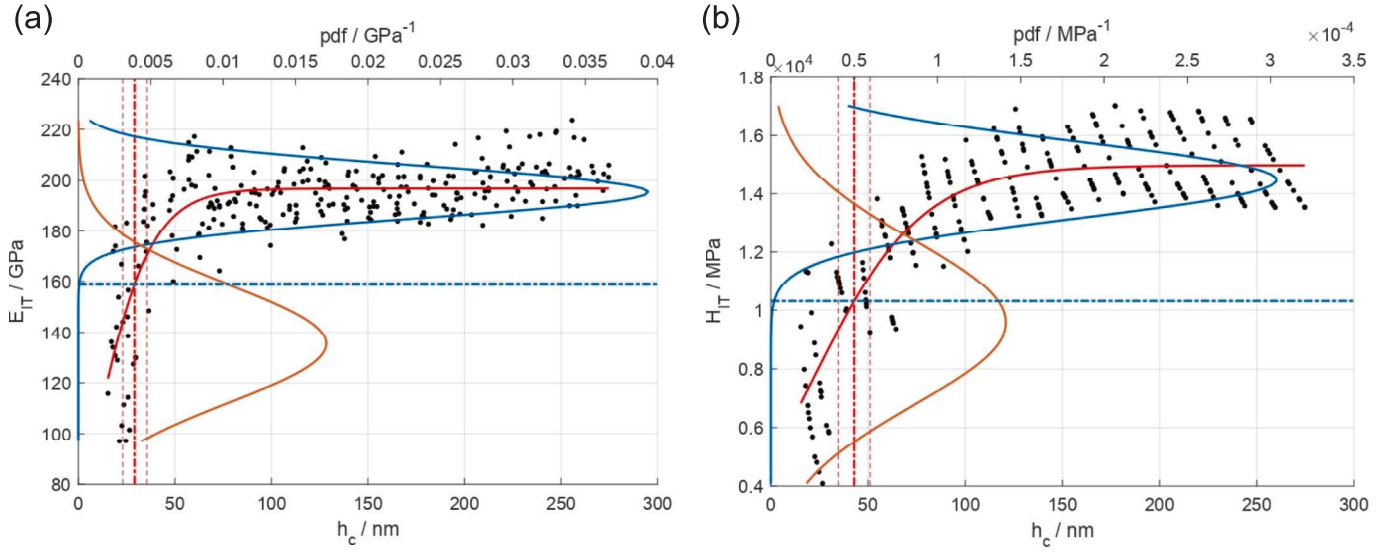
Fig. 6. Method application result for \text{ZrO}_2\text{AgNP}/\text{Si}\langle 1\ 0\ 0 \rangle with a deposition duration of 30'. Black points: measured data. Orange solid line: probability density function of the coating (transition layer) mechanical response. Blue solid line: probability density function of the substrate mechanical response. Red solid line: fitted M = g(h_c) . Blue dot-dashed line: M_2^* . Red dot-dashed line: t_c = t_{M,2}^* = g^{-1}(M_2^*) , with expanded uncertainty (95% confidence level) (red dashed lines). Deconvolution of (a) E_{IT} and (b) H_{IT} .
