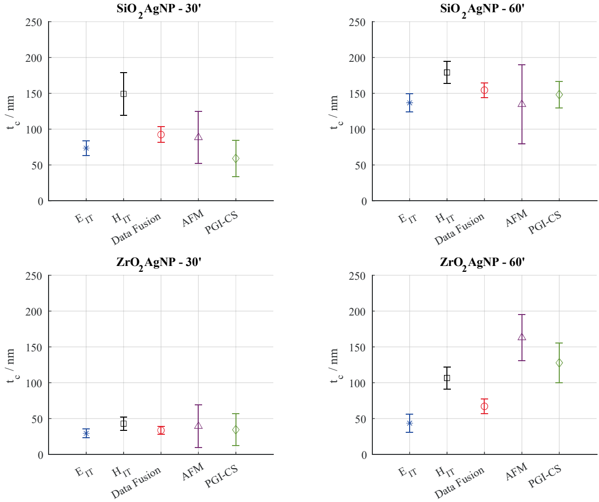
Fig. 8. Error bar plot with confidence interval at a 95% confidence level for the evaluated coating thickness (physical interface) based on nanoindentation-based method (using only the E_{IT} , the H_{IT} , or by Data fusion), and by directly traceable approaches, i.e. AFM and PGI-CS.
