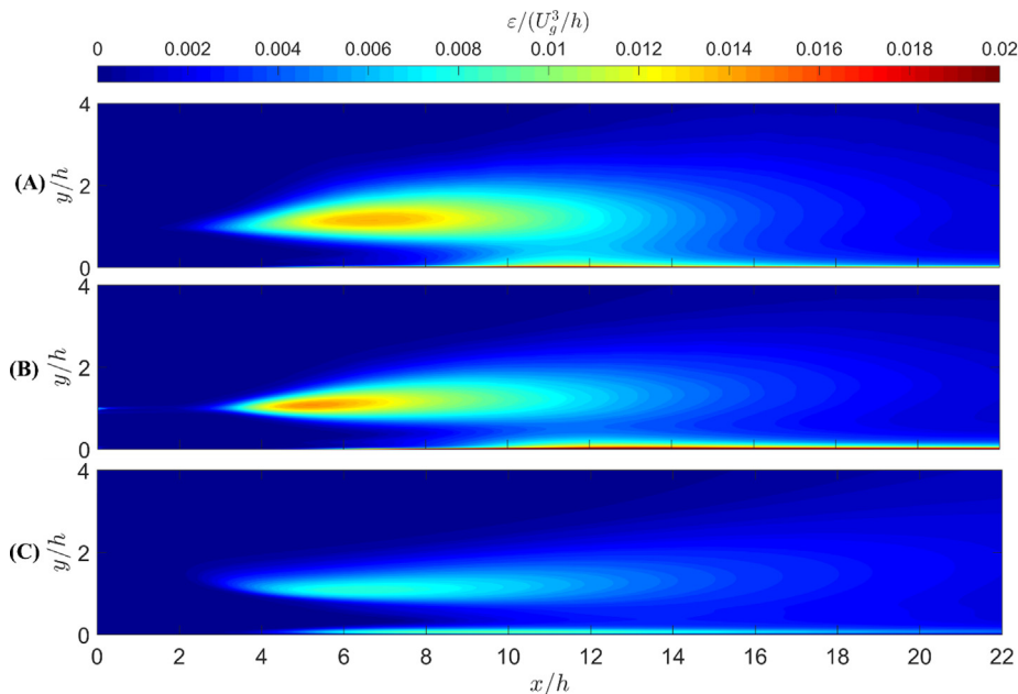
Fig. 8. Dissipation rate of TKE, \varepsilon , comparing validation data (DNS) (A) with the predictions obtained with the turbulence models: (B) LES and (C) RANS.
