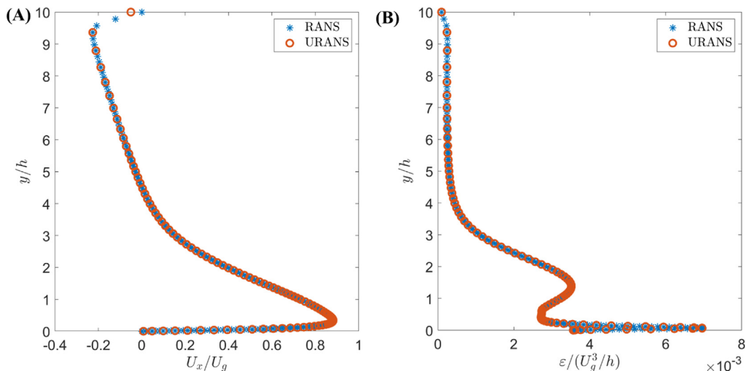
Fig. 11. Comparing (A) the average streamwise velocity, U_x , and (B) the dissipation rate of TKE, \varepsilon , as function of wallnormal distance, y , between RANS and URANS. ( x/h = 16 ).
