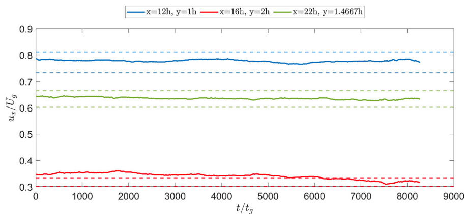
Fig. 3. Running average of streamwise velocity, u_x , at different points in the spanwise plane ( z/h = 1 ) with window size of 0.2 s (4300 t_g ). The horizontal axis shows the normalized time from the beginning of the simulation.
