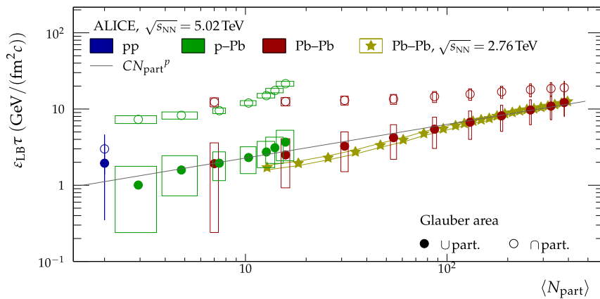
Fig. 6. Estimate of the lower bound on the Bjorken transverse energy density in pp, p-Pb, and Pb-Pb collisions at \sqrt{s_{NN}} = 5.02 TeV, considering the exclusive ( \square , open markers) and inclusive ( \blacksquare , full markers) overlap area S_T of the nucleons. The expression CN_{part}^p is fitted to case \square , and we find C = (0.8 \pm 0.3) GeV/( \text{fm}^2c ) and p = 0.44 \pm 0.08 . Also shown is an estimate, via dE_T/dy , of \varepsilon_{Bj} from Pb-Pb collisions at \sqrt{s_{NN}} = 2.76 TeV (stars with uncertainty band) [31].
