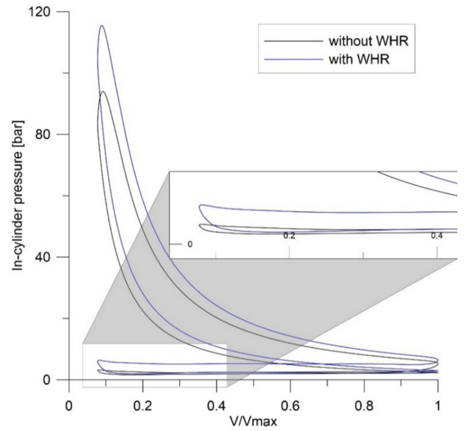
Fig. 8. Indicated cycles for a specific working point, with and without recovery sections in the exhausts.
