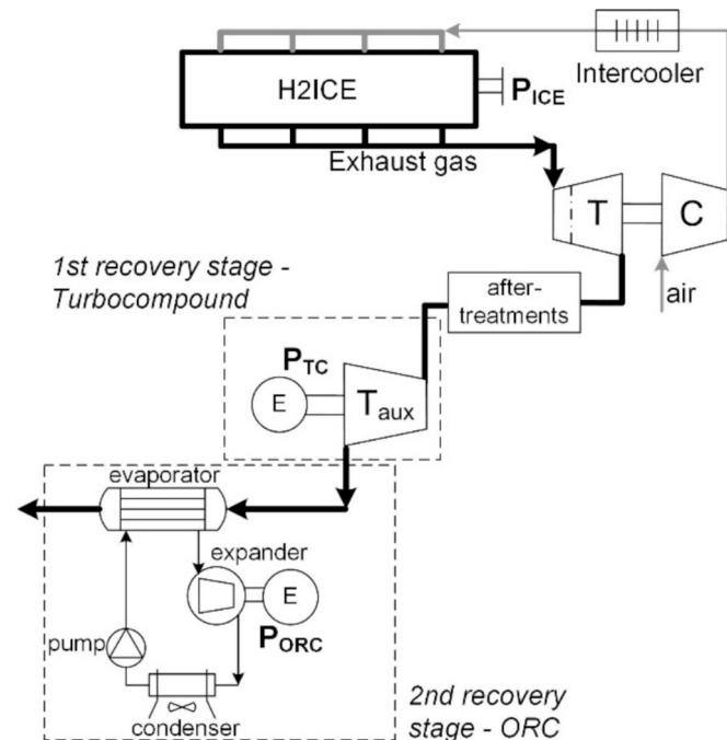
Fig. 6. Two-stage WHR recovery section considered.
