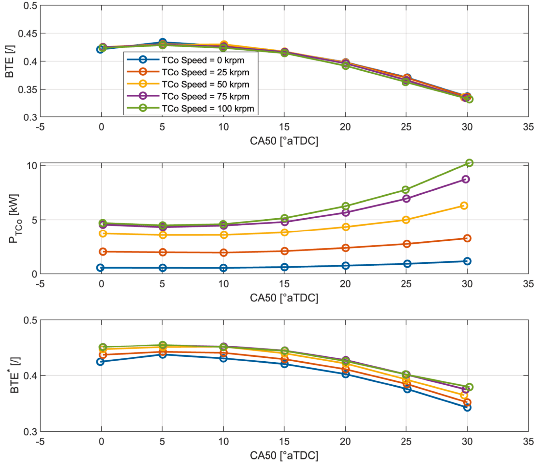
Fig. 13. BTE (top), PTC (middle) and \text{BTE}^* (bottom) for fixed engine speed, \lambda and different TC speeds.
