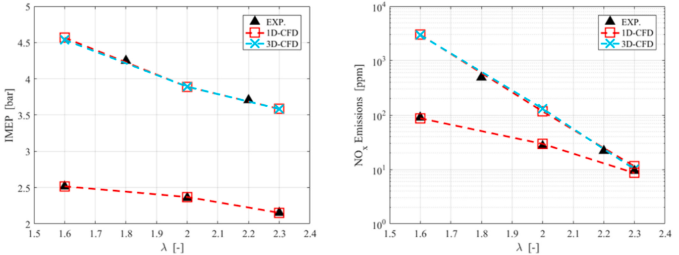
Fig. 5. Measured and simulated IMEP (left) and NO x emissions (right) for two lambda sweeps at different engine loads.
