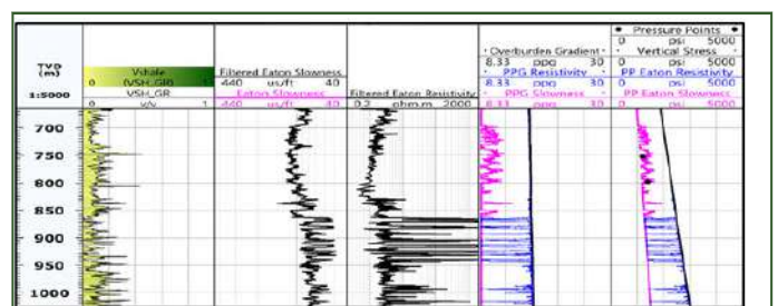
Figure 8: Pore pressure assessment with Eaton’s slowness logs.
