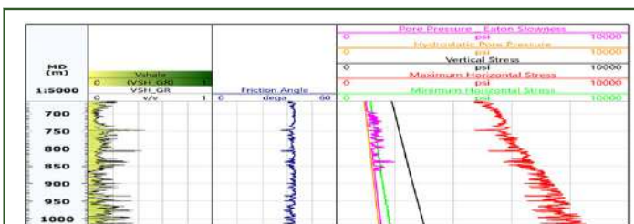
Figure 7: Horizontal stresses of dammam formation predicted according to the Mohr-Coulomb model.
