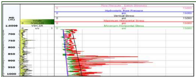
Figure 6: Horizontal stresses of Dammam formation predicted according to the poro elastic horizontal strain model.
