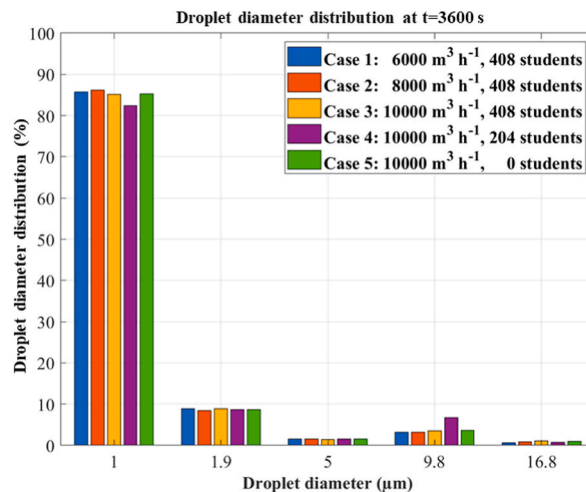
Fig. 11. Droplet distribution as function of the diameter, at the end of simulation ( t = 3600 s), for all the simulated cases.
