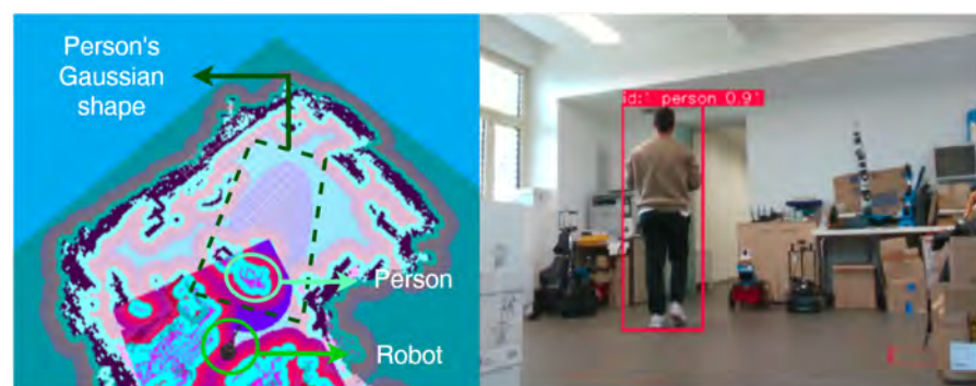
Figure 14. Safe navigation behavior of the mobile manipulator. (Left) RViz visualization of the person's Gaussian shape. (Right) Robot's point of view of the identified person.
