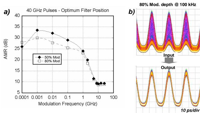
Fig. 9. (a). AMR vs. modulation frequency for 40 GHz pulse trains with 50 and 80% modulation depths. b) Input/output evolution of 80%-modulated pulse train (at 100 kHz modulation frequency).
