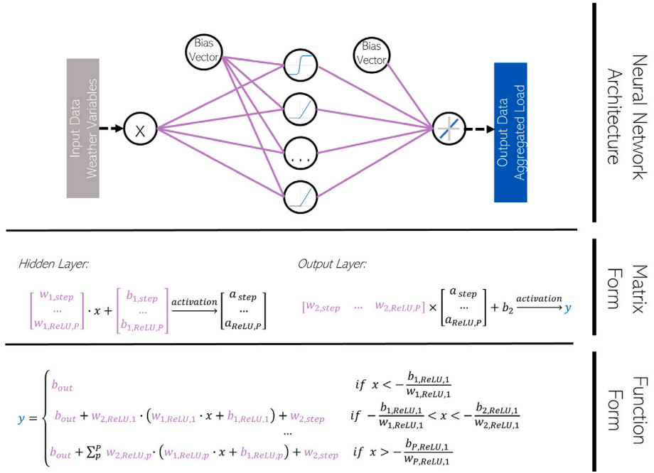
Fig. 3. Analogy of the human brain-inspired representation, the matrix form and the function form of an NN-based regression model.
