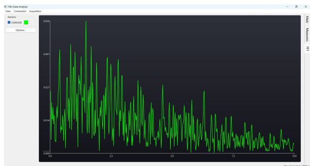
FIGURE 5. A screenshot of the FFT view of the PhotoNext FBG Data Analyzer .
