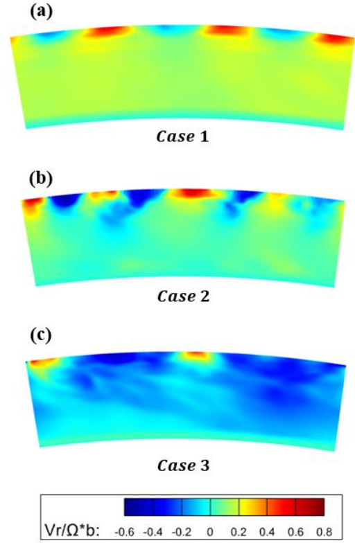
FIGURE 10: INSTANTANEOUS RADIAL VELOCITY CONTOURS FOR THE 16.875° SECTOR, CENTRAL PLANE: (a) C_w = 13110 ; (b) C_w = 2638 ; (c) C_w = -16747
