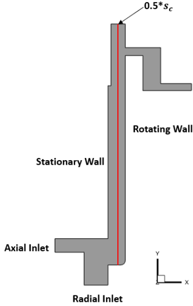
FIGURE 9: REFERENCE PLANE
