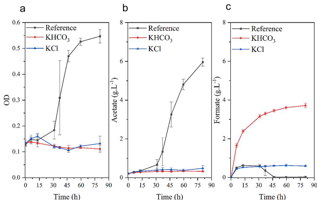
Fig. 9. Influence of the addition of 300 mM \text{KHCO}_3 or 300 mM KCl in the autotrophic medium. (a) T. kivui growth; (b) T. kivui acetate production; (c) T. kivui formic acid production. (Reference): bacteria growth in autotrophic medium without added salts.
