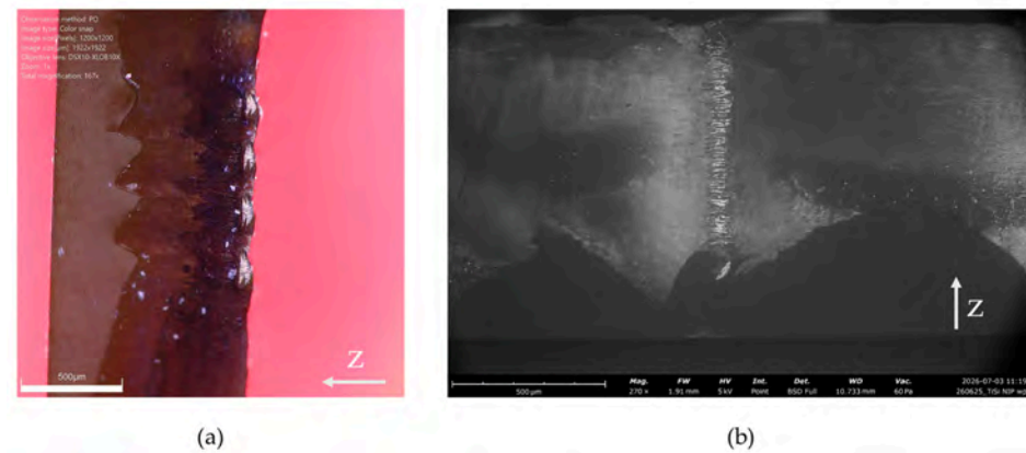
Figure 19. Hair effect as observed with (a) digital microscope; (b) SEM. In both pictures, the growth direction is highlighted.
