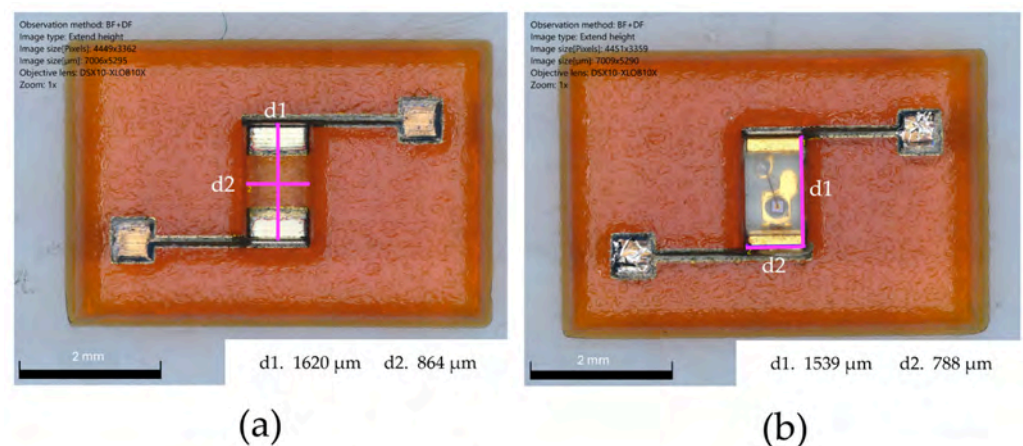
Figure 12. (a) Empty printed cavity; (b) cavity with the soldered component.
