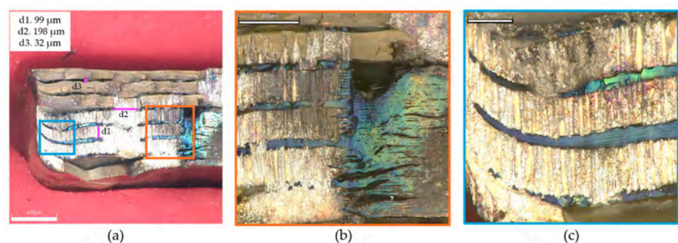
Figure 17. (a) Side view of the multilayered device; (b) detail of the interface between the layers and the dielectric substrate; (c) detail of the dielectric layers.
