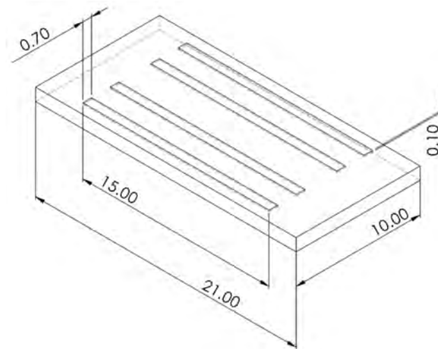
Figure 10. Model 7: conductive traces for electrical measurements. All measurements are in mm.
