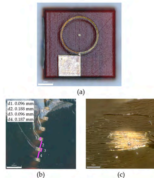
Figure 18. (a) Top view of Model 6; (b) side view of the internal structure of the device; (c) detail of one of the turns of the coil.
