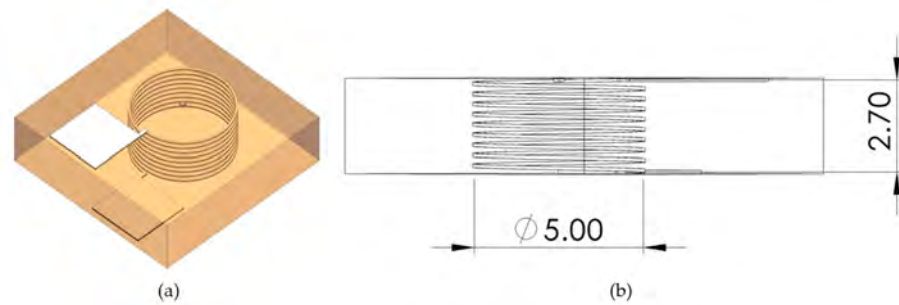
Figure 9. (a) Three-dimensional view and (b) side view of Model 6. All measurements are in mm.
