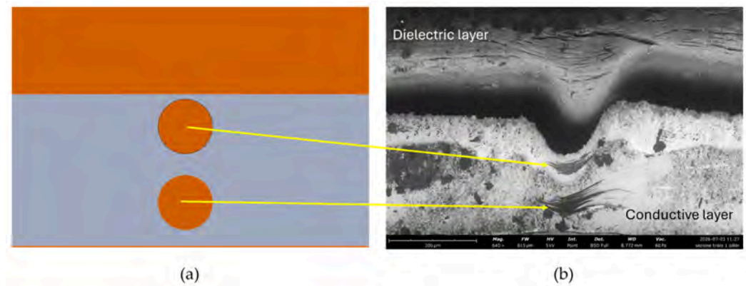
Figure 15. Comparison between (a) CAD model and (b) SEM cross-section of the channel, showing the dielectric pillars and the absence of a conductive layer after the second pillar.
