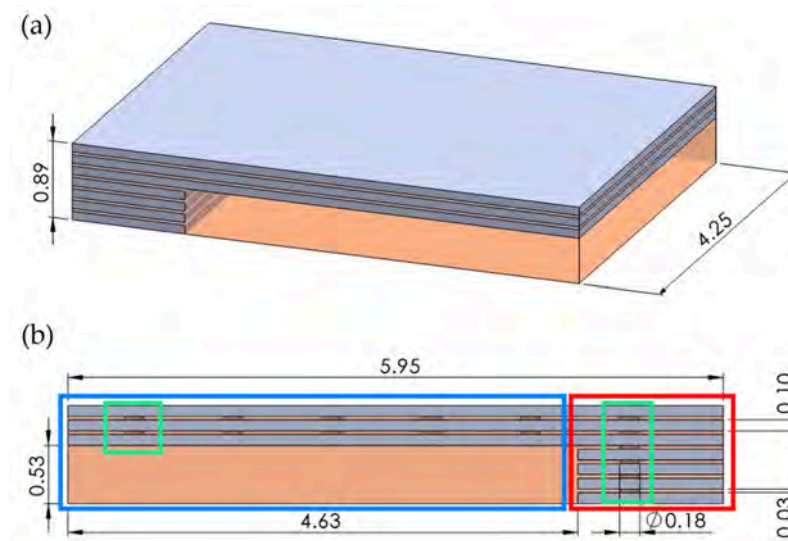
Figure 8. (a) Three-dimensional view and (b) side view of Model 5. In red, the portions of the device intended to act as terminals are indicated. In blue, the portion of the device intended to serve as a pad is indicated. In green, the vias that were used to connect the layers are indicated. All measurements are in mm.
