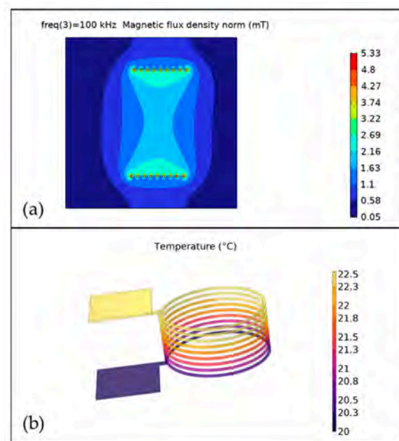
Figure 20. Results of the COMSOL simulations: (a) magnetic flux density norm of the device for f = 100 kHz; (b) graph of the temperatures reached on the solenoid.
