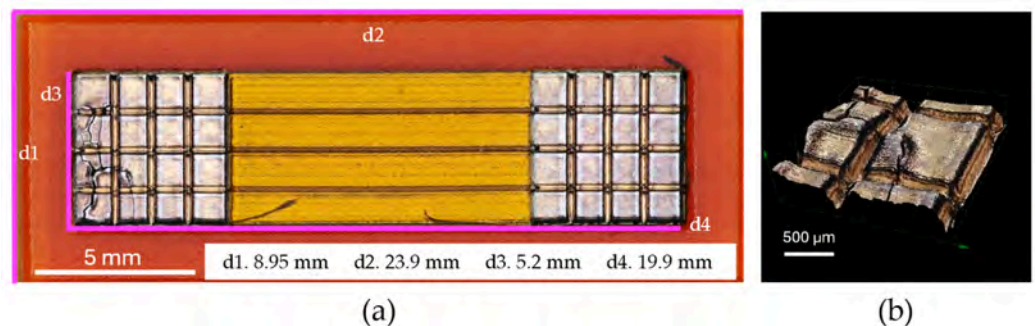
Figure 14. (a) Top view of Model 4; (b) 3D profile of the fractured surface of the pad at the bottom left.
