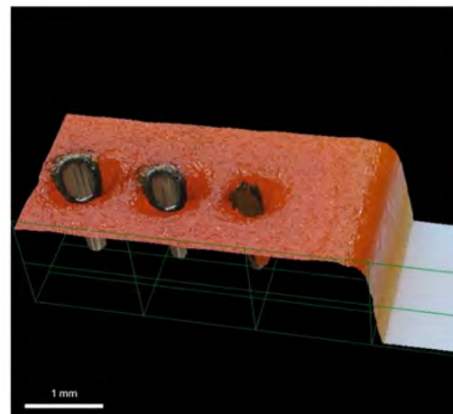
Figure 11. PTH profile. Via walls are sloped and cone-shaped.
