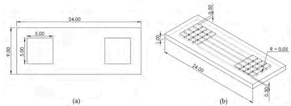
Figure 7. Model 4: (a) top view and (b) 3D view of the pads and a trace sample. Dashed lines represent pillars. All measurements are in mm.
