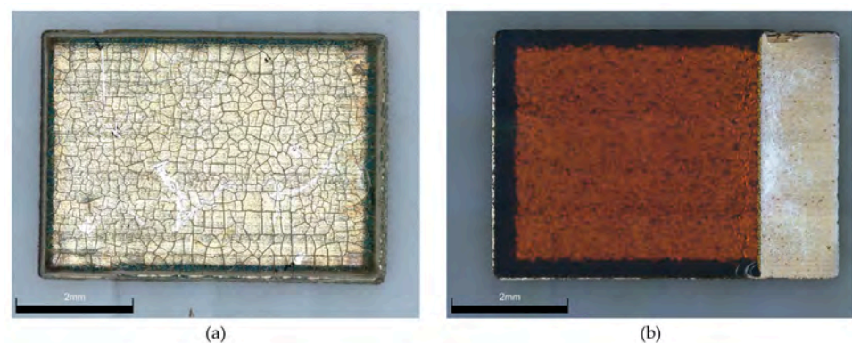
Figure 16. Printed Model 5. (a) Top view; (b) bottom-view of the multilayered device.
