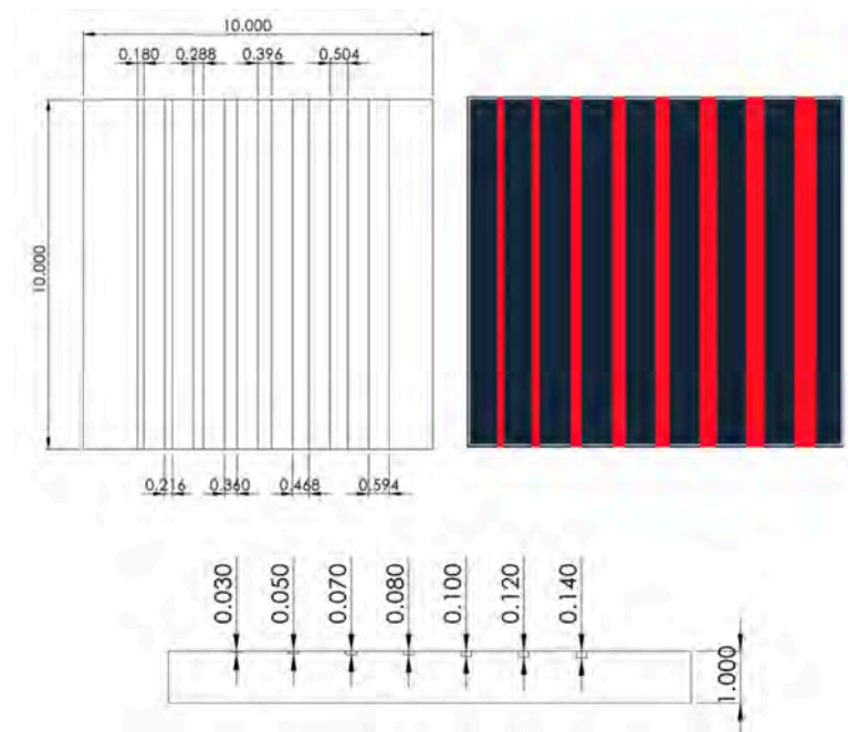
Figure 4. Model 1: (a) parallel trace design in SolidWorks and (b) KiCad, with dielectric material (dark blue) and conductive traces (red); (c) side view of the trace design in SolidWorks. All measurements are in mm.
