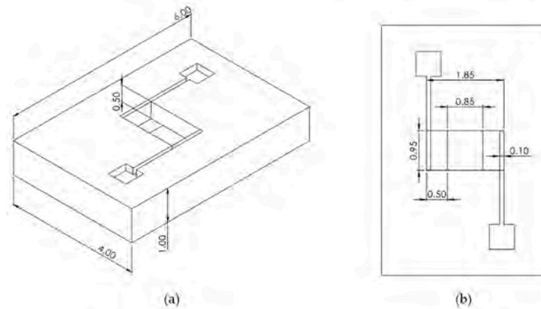
Figure 6. Model 3: (a) 3D view of the cavity design; (b) upper view of the cavity design. All measurements are in mm.
