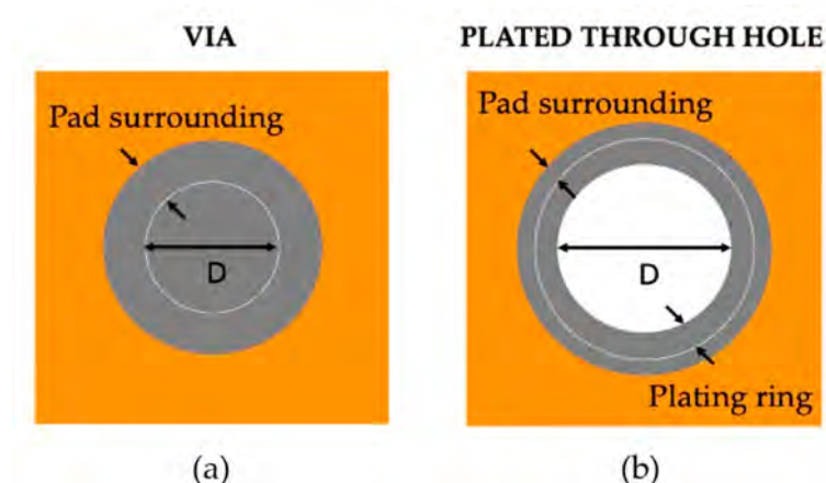
Figure 2. (a) Definition of pad surrounding for vias; (b) definition of plated ring for PTH.
