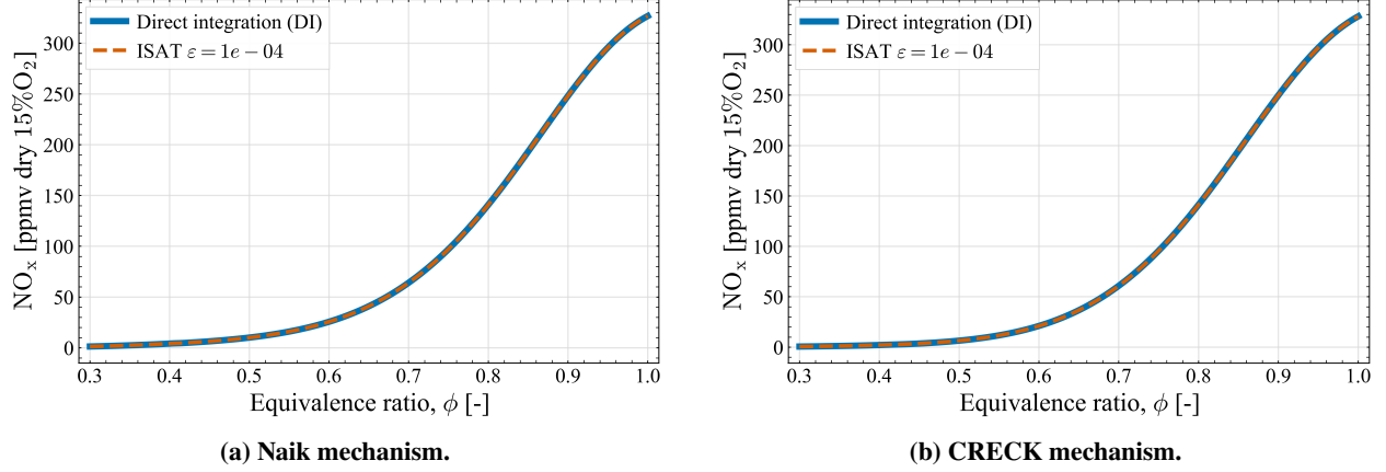
Fig. 8 \text{NO}_x emission as a function of equivalence ratio at \dot{m}_{\text{air}} = 130 \text{ kg/h} and T_{\text{air}} = 623 \text{ K} , predicted by direct integration and by the Flow-Map ISAT formulation at \varepsilon_{\text{tol}} = 10^{-4} .
