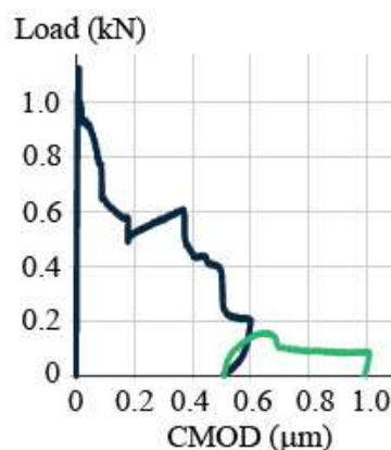
Fig. 7. Example of a load vs CMOD curve resulting from pre-loading (black curve) and re-loading (green curve) stages for a sample with a coated capsule.
