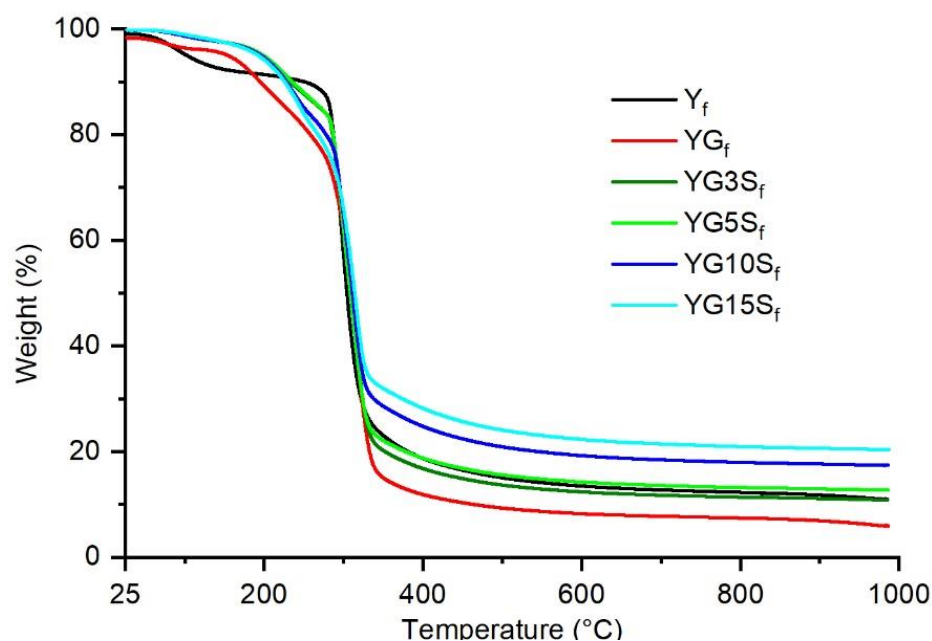
Figure 11. Thermograms of starch film ( Y_f ), plasticized starch film ( YG_f ) and nanocomposite films with different loadings of sepiolite ( YG3S_f , YG5S_f , YG10S_f and YG15S_f ).
